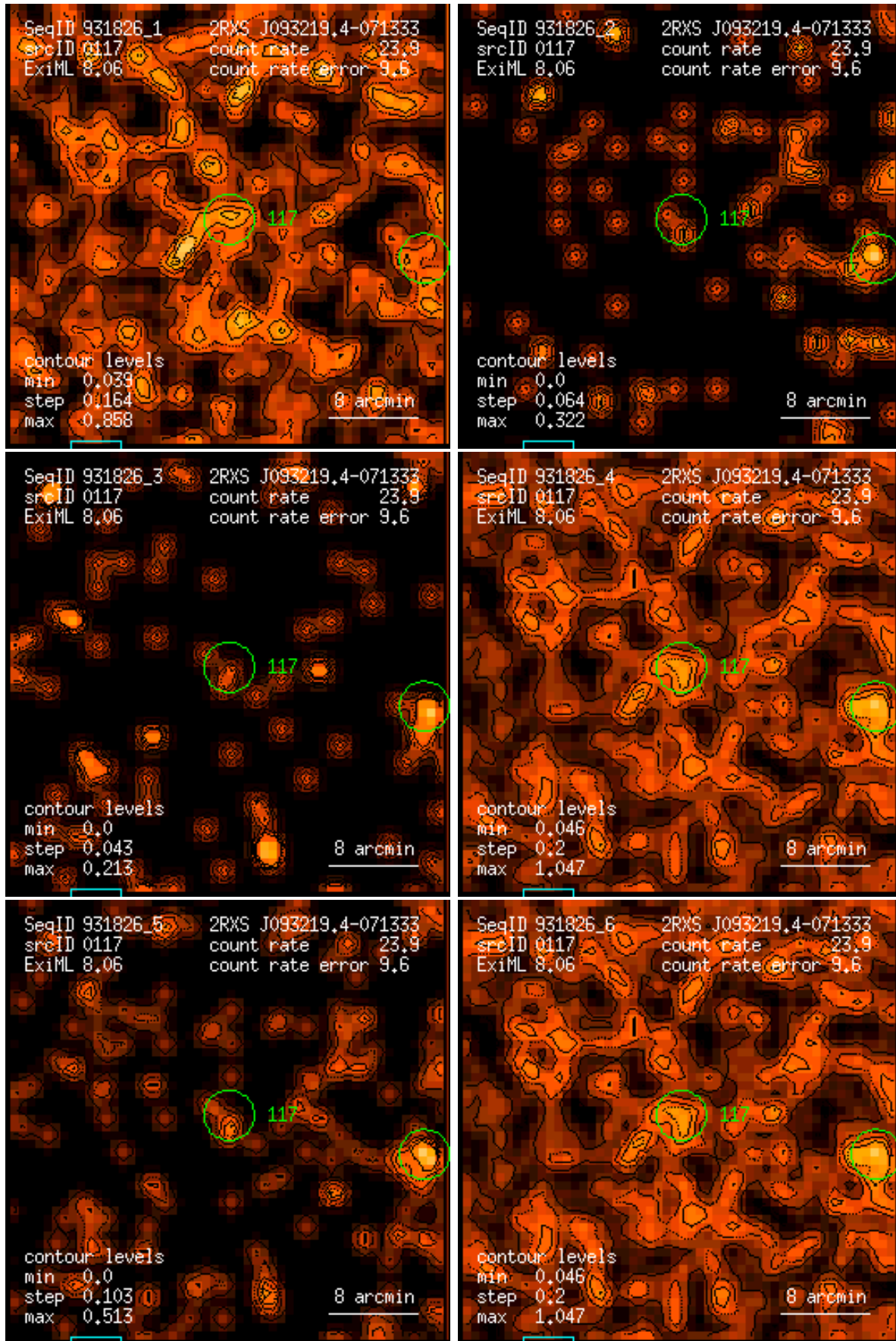
Figure 117: RASS 931826: detection 0117: band rate images, Gaussian filter: (1) PSPC channels 11 – 41, (2) 52 – 90, (3) 91 – 201, (4) 11 – 235, (5) 52 – 201, (6) 11 – 201. Broad band rates in counts/ks. Band rate contour levels in counts/ks/arcmin 2 .
