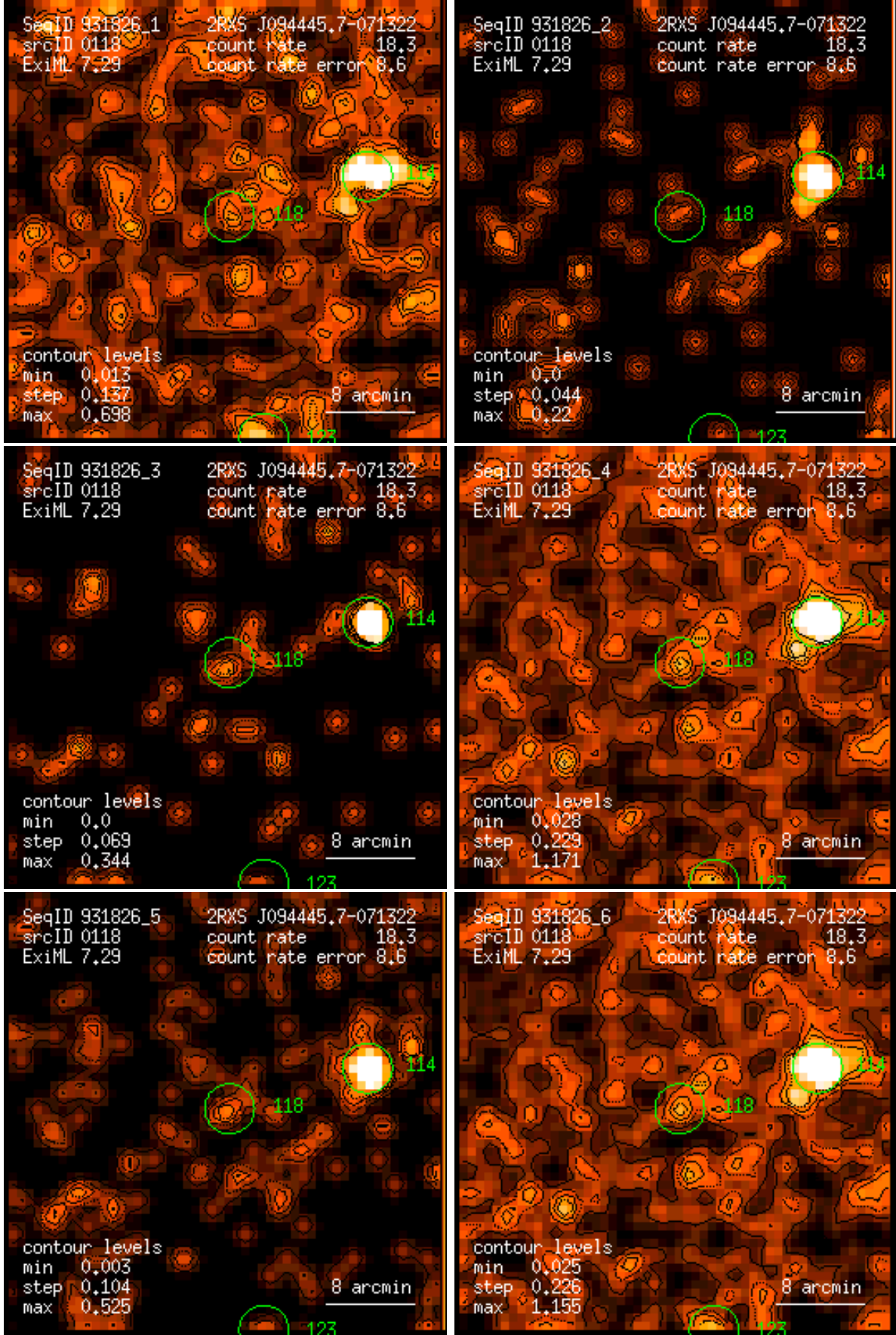
Figure 118: RASS 931826: detection 0118: band rate images, Gaussian filter: (1) PSPC channels 11 – 41, (2) 52 – 90, (3) 91 – 201, (4) 11 – 235, (5) 52 – 201, (6) 11 – 201. Broad band rates in counts/ks. Band rate contour levels in counts/ks/arcmin 2 .
