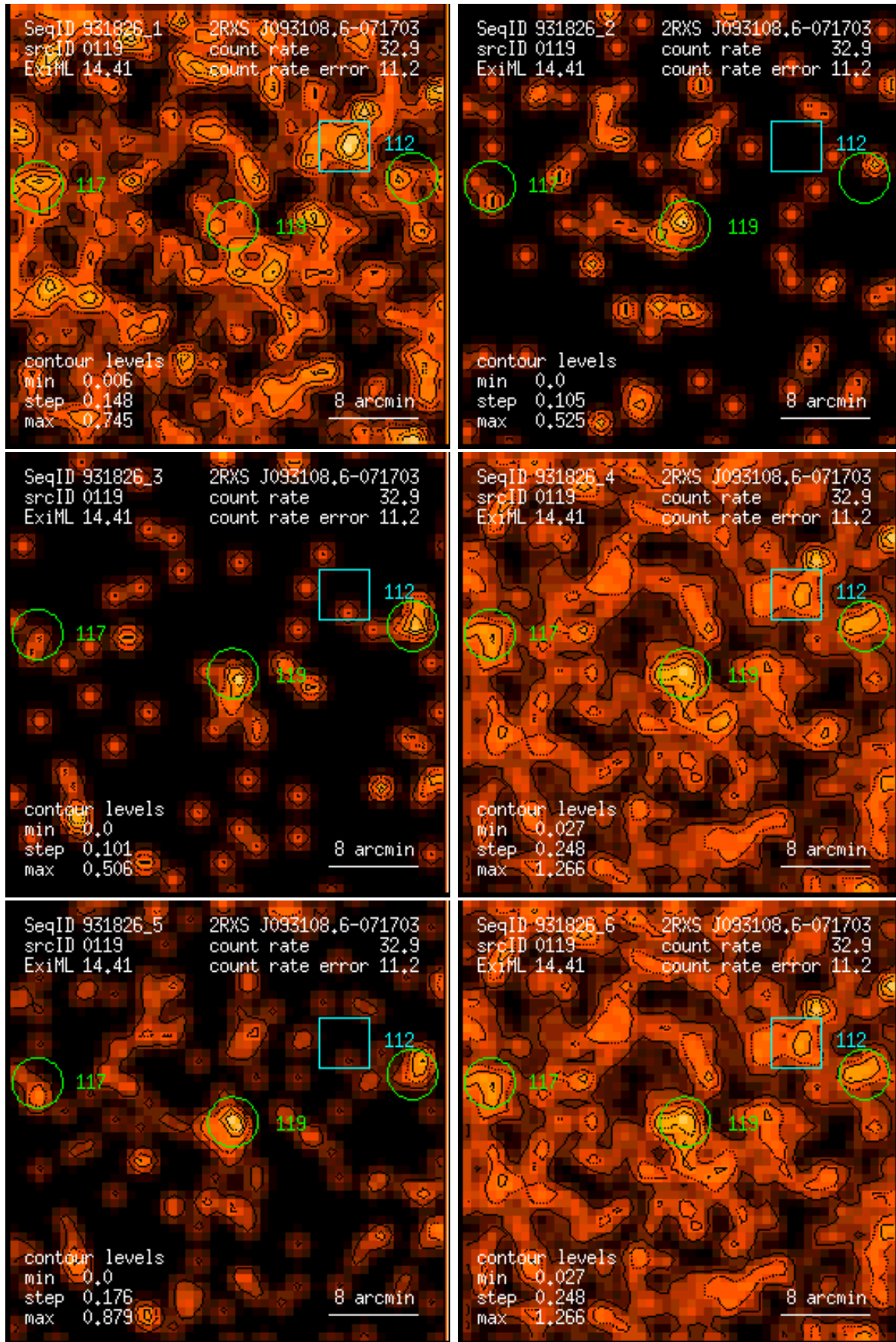
Figure 119: RASS 931826: detection 0119: band rate images, Gaussian filter: (1) PSPC channels 11 – 41, (2) 52 – 90, (3) 91 – 201, (4) 11 – 235, (5) 52 – 201, (6) 11 – 201. Broad band rates in counts/ks. Band rate contour levels in counts/ks/arcmin 2 .
