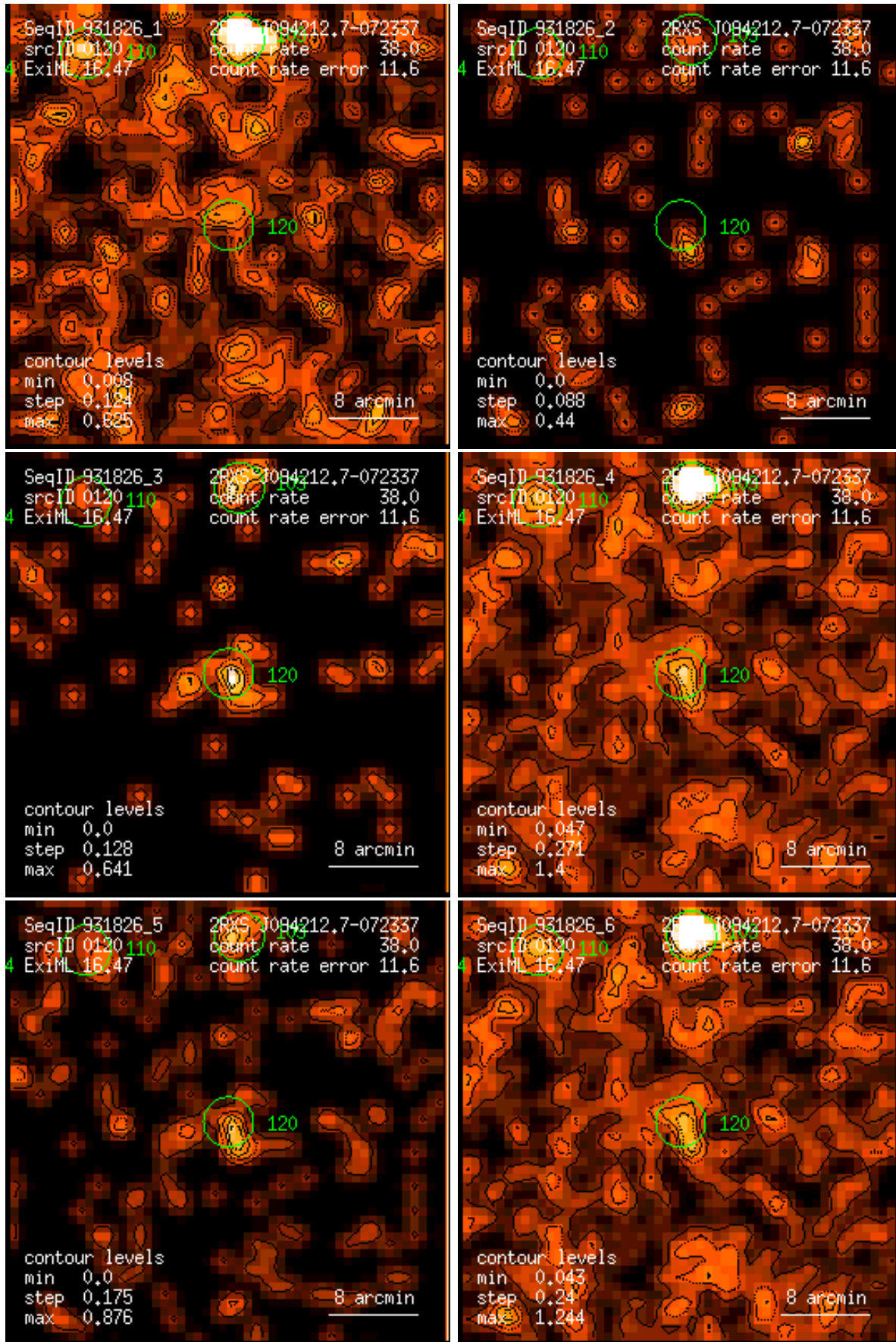
Figure 120: RASS 931826: detection 0120: band rate images, Gaussian filter: (1) PSPC channels 11 – 41, (2) 52 – 90, (3) 91 – 201, (4) 11 – 235, (5) 52 – 201, (6) 11 – 201. Broad band rates in counts/ks. Band rate contour levels in counts/ks/arcmin 2 .
