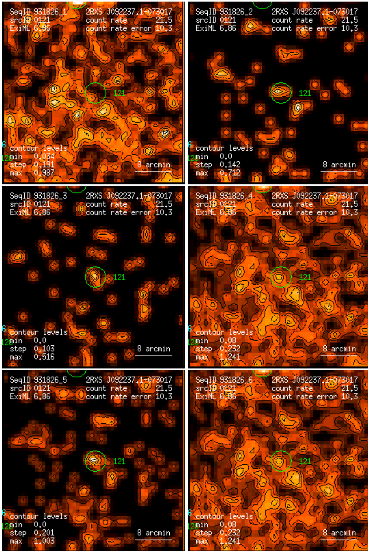
Figure 121: RASS 931826: detection 0121: band rate images, Gaussian filter: (1) PSPC channels 11 – 41, (2) 52 – 90, (3) 91 – 201, (4) 11 – 235, (5) 52 – 201, (6) 11 – 201. Broad band rates in counts/ks. Band rate contour levels in counts/ks/arcmin 2 .
