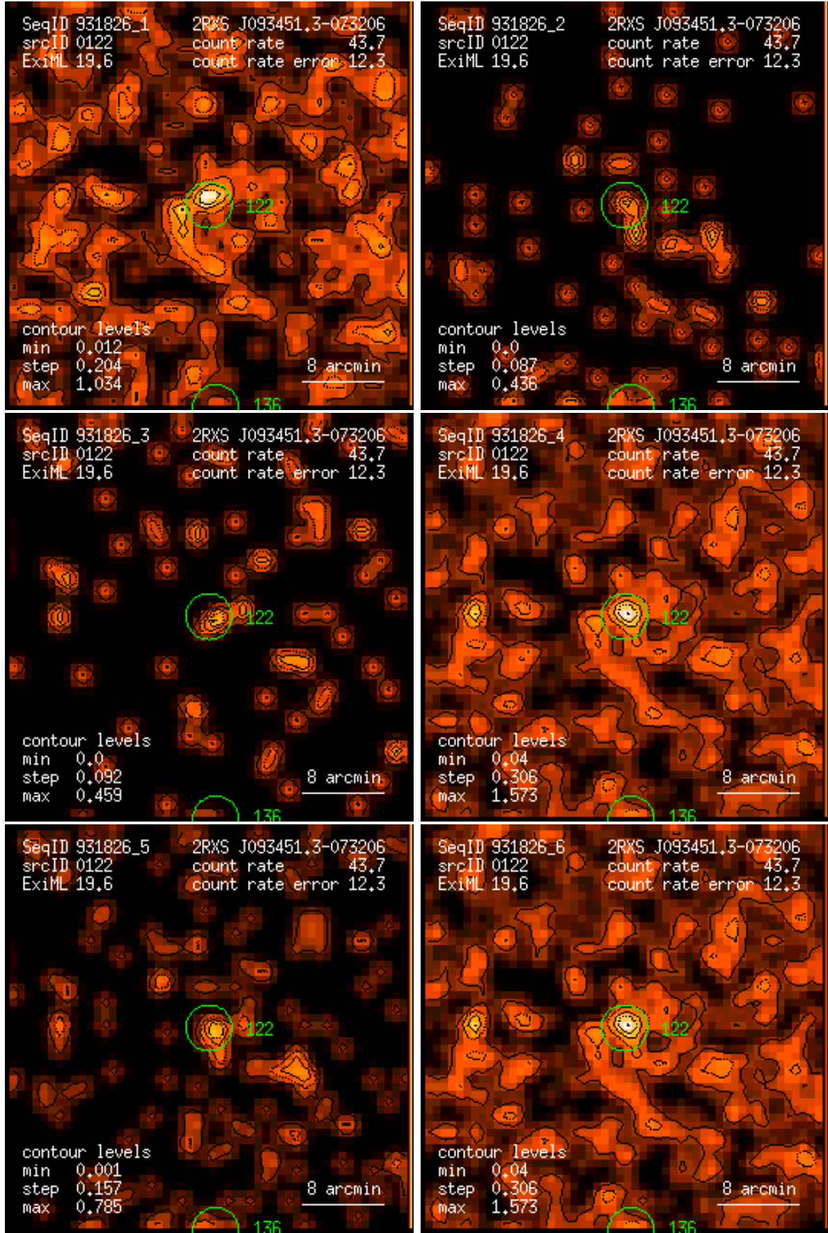
Figure 122: RASS 931826: detection 0122: band rate images, Gaussian filter: (1) PSPC channels 11 – 41, (2) 52 – 90, (3) 91 – 201, (4) 11 – 235, (5) 52 – 201, (6) 11 – 201. Broad band rates in counts/ks. Band rate contour levels in counts/ks/arcmin 2 .
