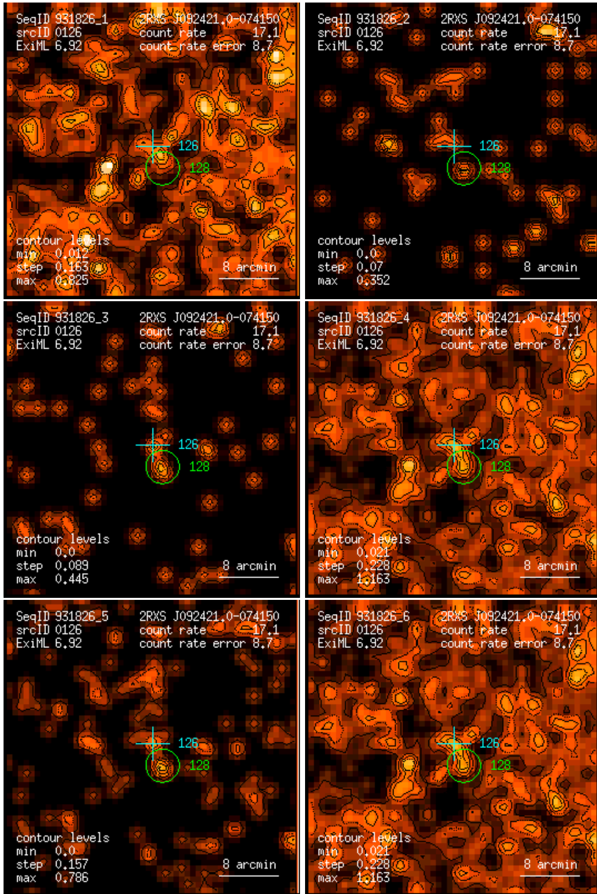
Figure 126: RASS 931826: detection 0126: band rate images, Gaussian filter: (1) PSPC channels 11 – 41, (2) 52 – 90, (3) 91 – 201, (4) 11 – 235, (5) 52 – 201, (6) 11 – 201. Broad band rates in counts/ks. Band rate contour levels in counts/ks/arcmin 2 .
