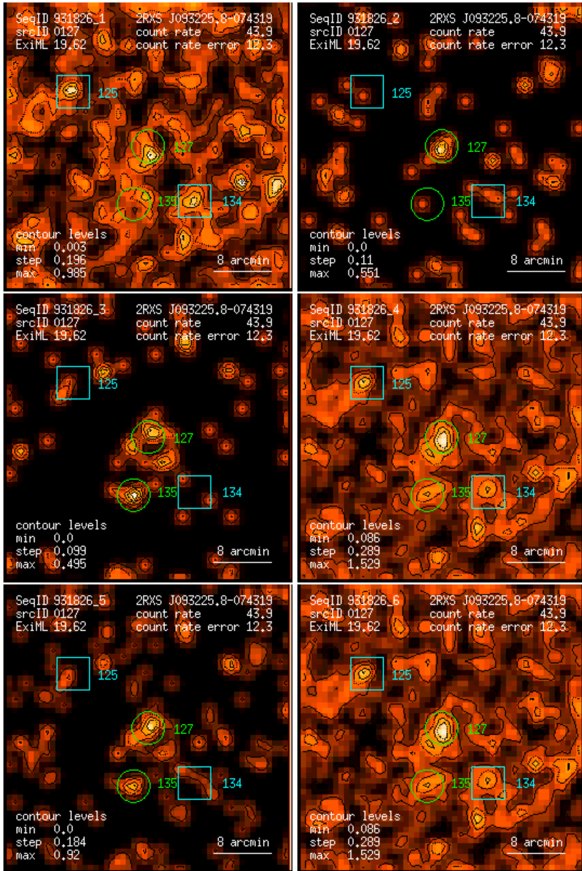
Figure 127: RASS 931826: detection 0127: band rate images, Gaussian filter: (1) PSPC channels 11 – 41, (2) 52 – 90, (3) 91 – 201, (4) 11 – 235, (5) 52 – 201, (6) 11 – 201. Broad band rates in counts/ks. Band rate contour levels in counts/ks/arcmin 2 .
