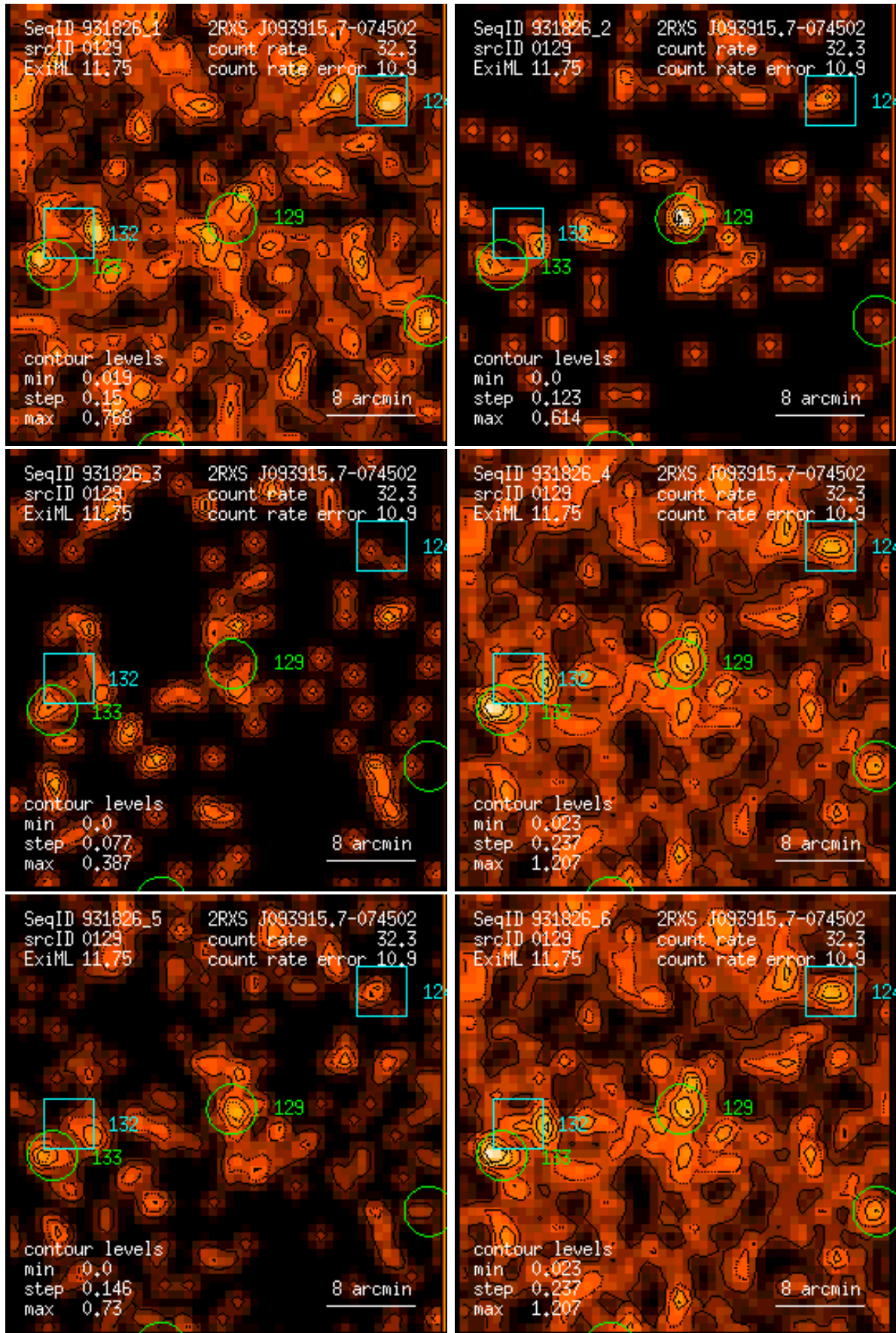
Figure 129: RASS 931826: detection 0129: band rate images, Gaussian filter: (1) PSPC channels 11 – 41, (2) 52 – 90, (3) 91 – 201, (4) 11 – 235, (5) 52 – 201, (6) 11 – 201. Broad band rates in counts/ks. Band rate contour levels in counts/ks/arcmin 2 .
