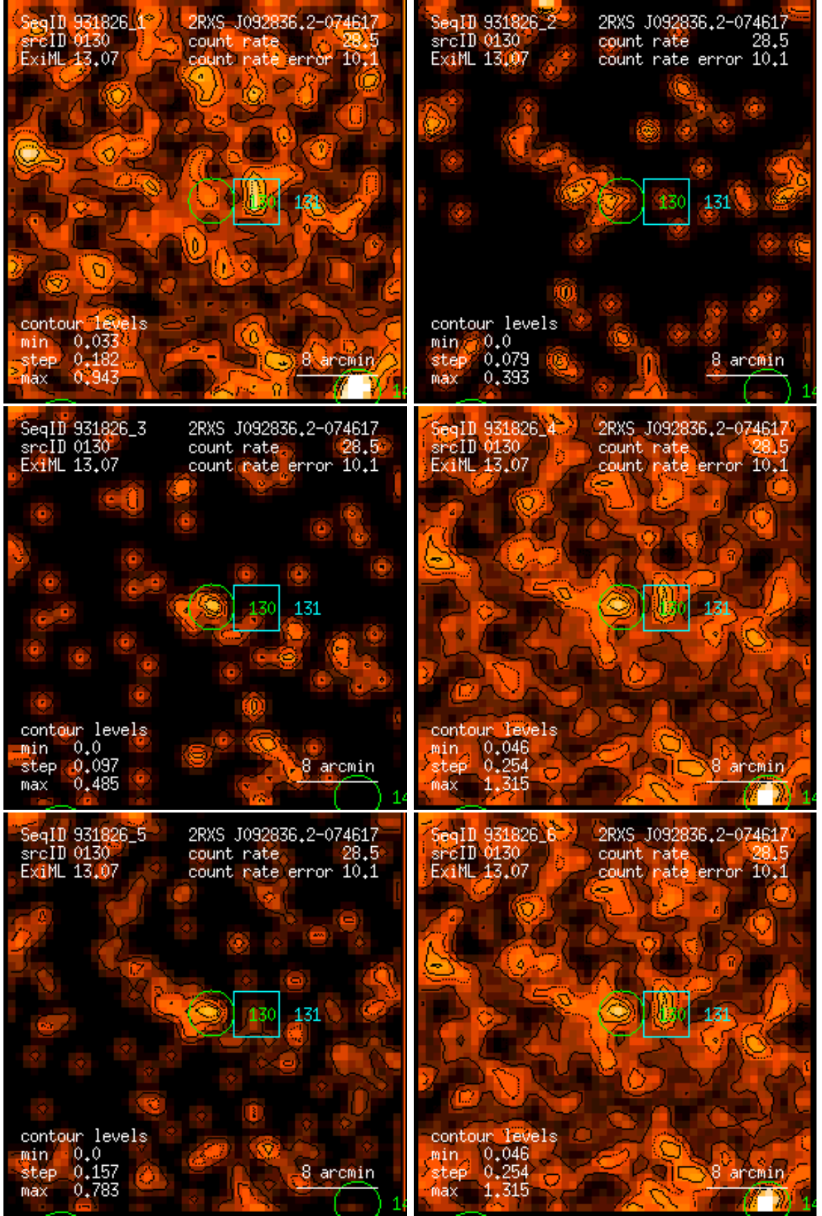
Figure 130: RASS 931826: detection 0130: band rate images, Gaussian filter: (1) PSPC channels 11 – 41, (2) 52 – 90, (3) 91 – 201, (4) 11 – 235, (5) 52 – 201, (6) 11 – 201. Broad band rates in counts/ks. Band rate contour levels in counts/ks/arcmin 2 .
