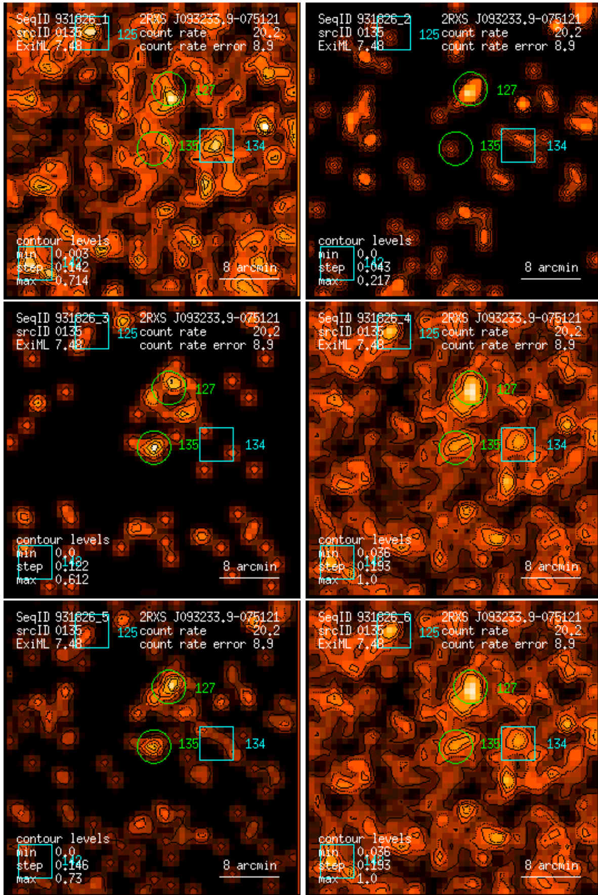
Figure 135: RASS 931826: detection 0135: band rate images, Gaussian filter: (1) PSPC channels 11 – 41, (2) 52 – 90, (3) 91 – 201, (4) 11 – 235, (5) 52 – 201, (6) 11 – 201. Broad band rates in counts/ks. Band rate contour levels in counts/ks/arcmin 2 .
