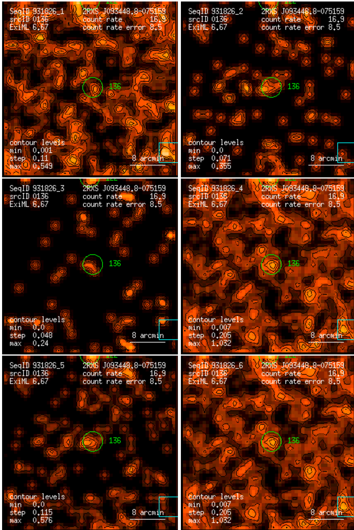
Figure 136: RASS 931826: detection 0136: band rate images, Gaussian filter: (1) PSPC channels 11 – 41, (2) 52 – 90, (3) 91 – 201, (4) 11 – 235, (5) 52 – 201, (6) 11 – 201. Broad band rates in counts/ks. Band rate contour levels in counts/ks/arcmin 2 .
