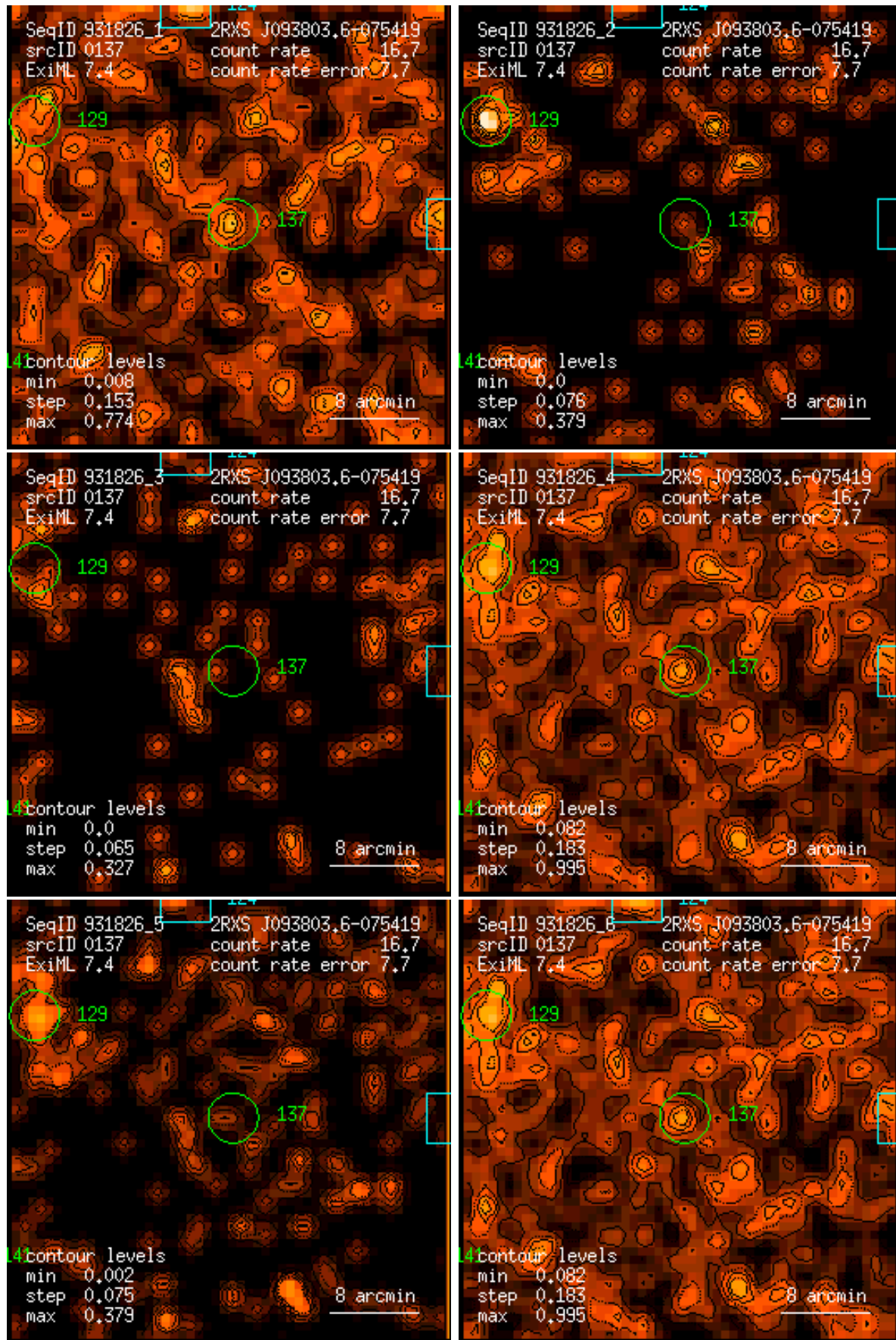
Figure 137: RASS 931826: detection 0137: band rate images, Gaussian filter: (1) PSPC channels 11 – 41, (2) 52 – 90, (3) 91 – 201, (4) 11 – 235, (5) 52 – 201, (6) 11 – 201. Broad band rates in counts/ks. Band rate contour levels in counts/ks/arcmin 2 .
