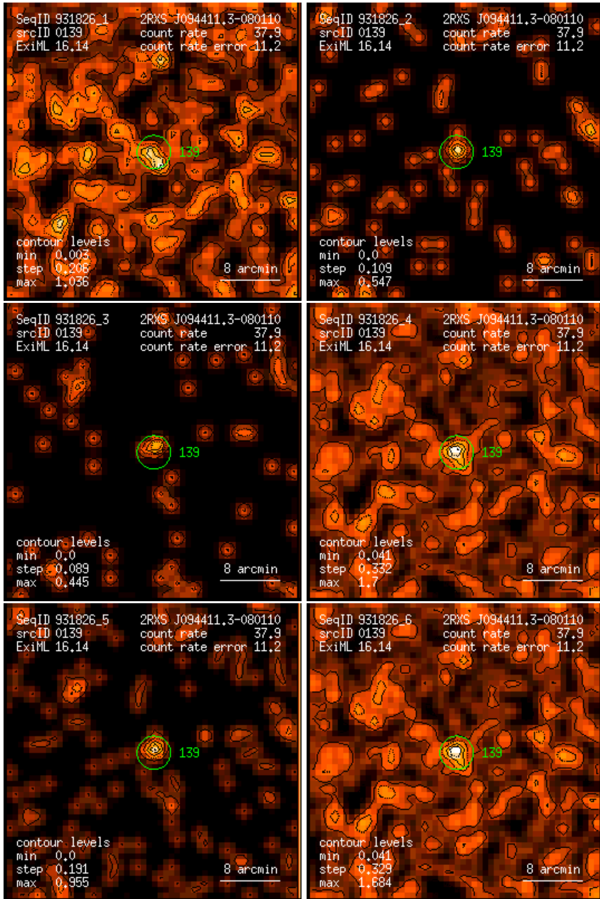
Figure 139: RASS 931826: detection 0139: band rate images, Gaussian filter: (1) PSPC channels 11 – 41, (2) 52 – 90, (3) 91 – 201, (4) 11 – 235, (5) 52 – 201, (6) 11 – 201. Broad band rates in counts/ks. Band rate contour levels in counts/ks/arcmin 2 .
