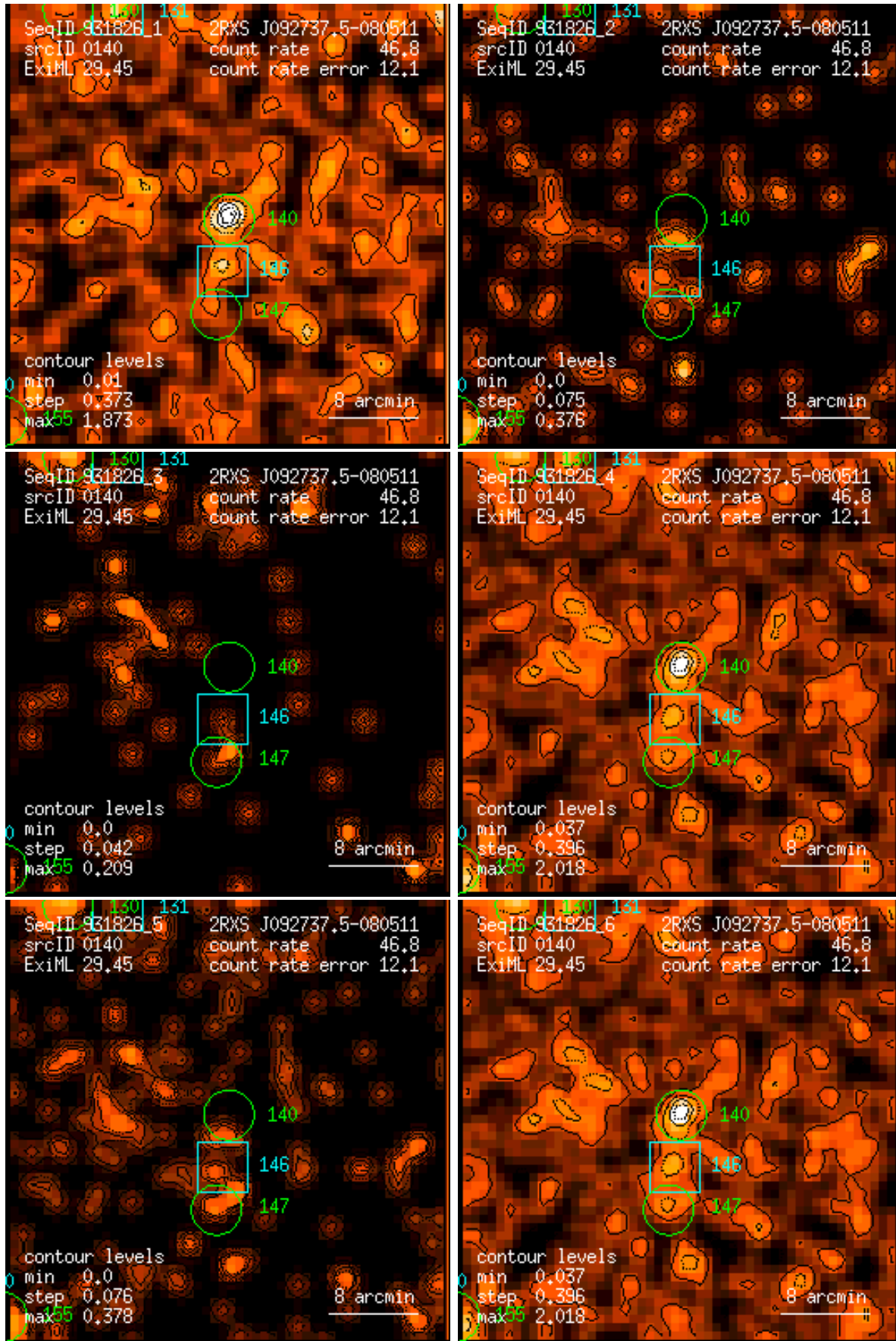
Figure 140: RASS 931826: detection 0140: band rate images, Gaussian filter: (1) PSPC channels 11 – 41, (2) 52 – 90, (3) 91 – 201, (4) 11 – 235, (5) 52 – 201, (6) 11 – 201. Broad band rates in counts/ks. Band rate contour levels in counts/ks/arcmin 2 .
