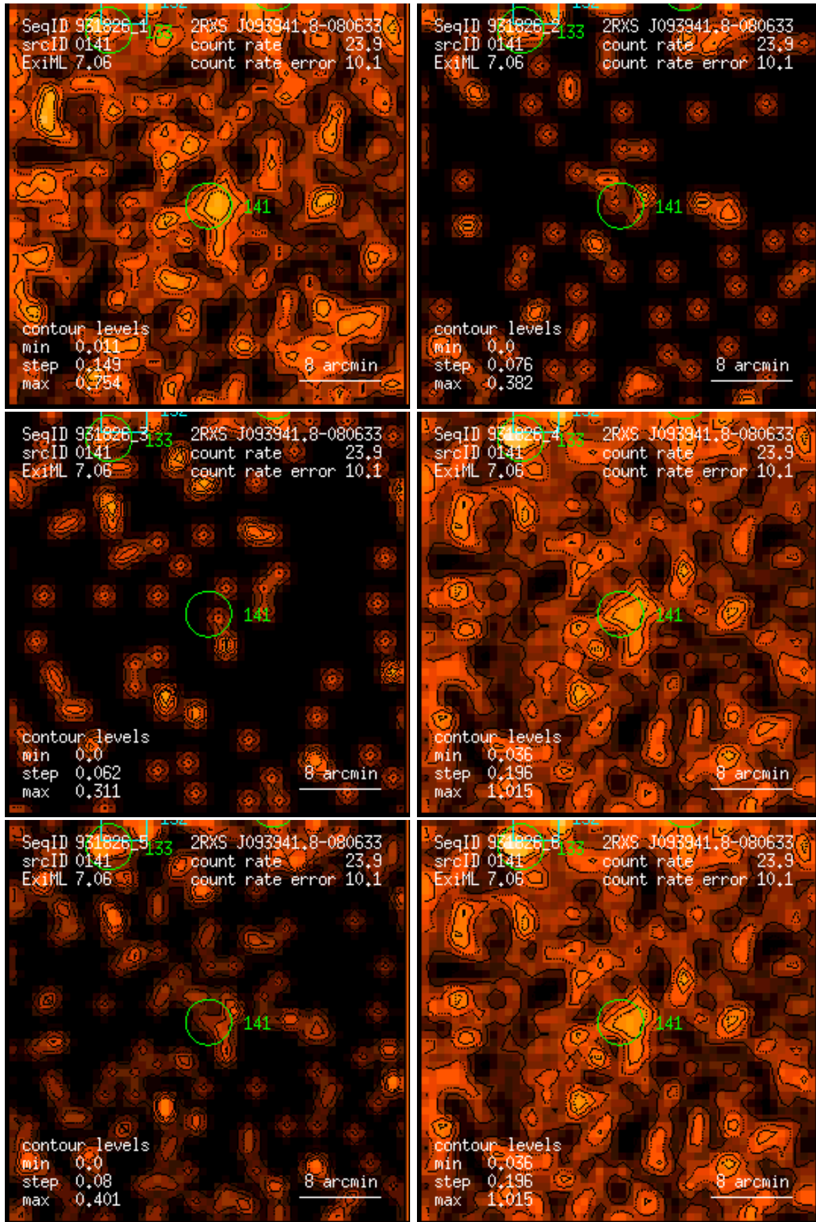
Figure 141: RASS 931826: detection 0141: band rate images, Gaussian filter: (1) PSPC channels 11 – 41, (2) 52 – 90, (3) 91 – 201, (4) 11 – 235, (5) 52 – 201, (6) 11 – 201. Broad band rates in counts/ks. Band rate contour levels in counts/ks/arcmin 2 .
