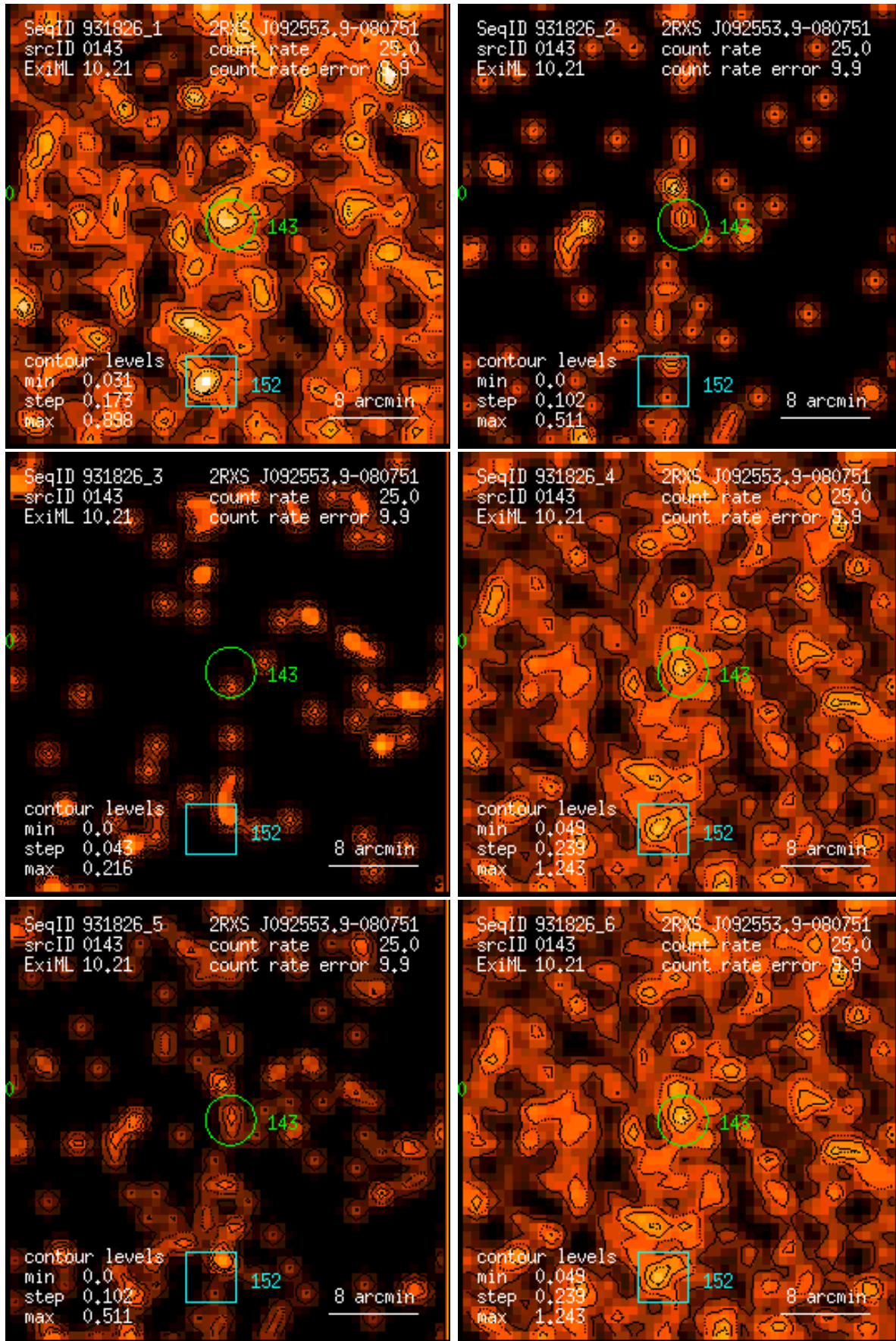
Figure 143: RASS 931826: detection 0143: band rate images, Gaussian filter: (1) PSPC channels 11 – 41, (2) 52 – 90, (3) 91 – 201, (4) 11 – 235, (5) 52 – 201, (6) 11 – 201. Broad band rates in counts/ks. Band rate contour levels in counts/ks/arcmin 2 .
