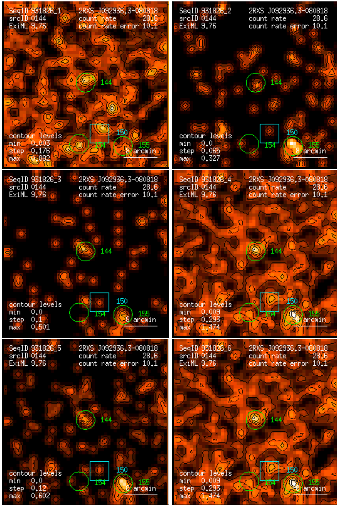
Figure 144: RASS 931826: detection 0144: band rate images, Gaussian filter: (1) PSPC channels 11 – 41, (2) 52 – 90, (3) 91 – 201, (4) 11 – 235, (5) 52 – 201, (6) 11 – 201. Broad band rates in counts/ks. Band rate contour levels in counts/ks/arcmin 2 .
