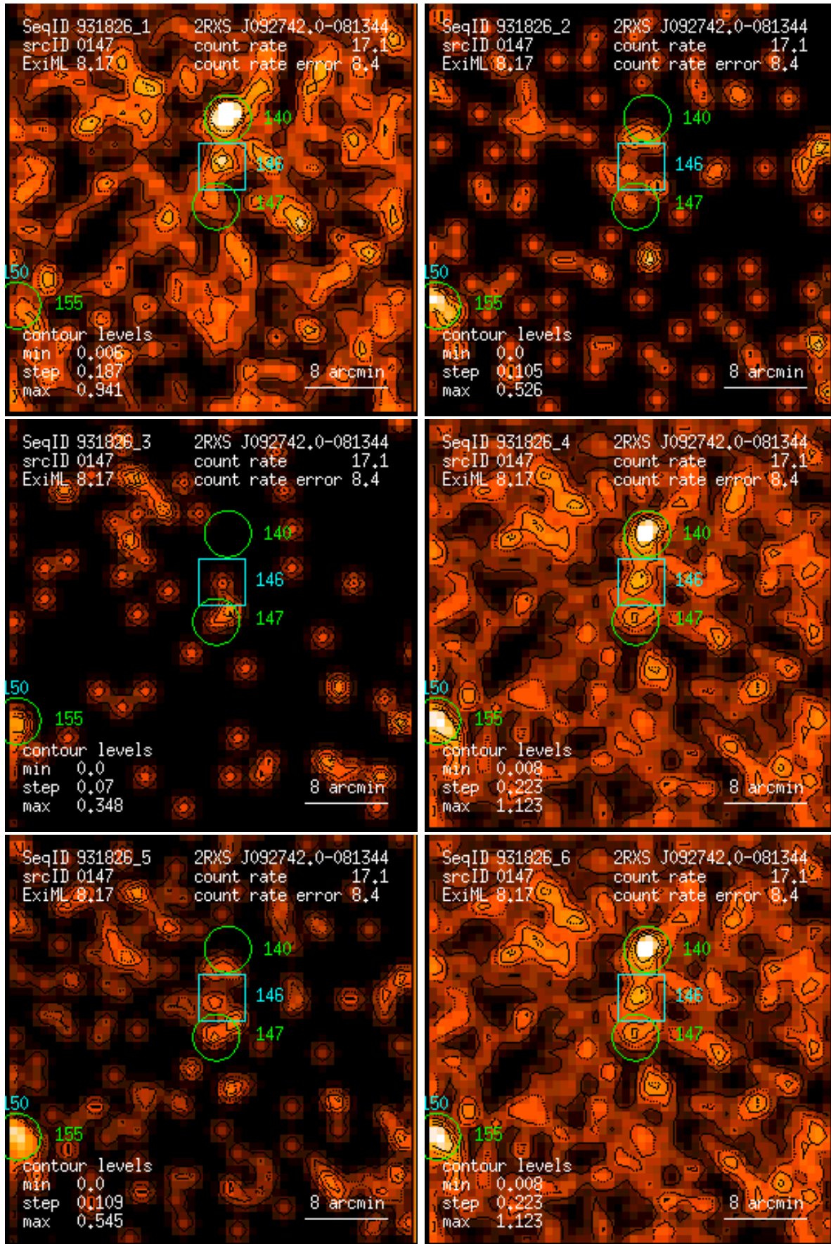
Figure 147: RASS 931826: detection 0147: band rate images, Gaussian filter: (1) PSPC channels 11 – 41, (2) 52 – 90, (3) 91 – 201, (4) 11 – 235, (5) 52 – 201, (6) 11 – 201. Broad band rates in counts/ks. Band rate contour levels in counts/ks/arcmin 2 .
