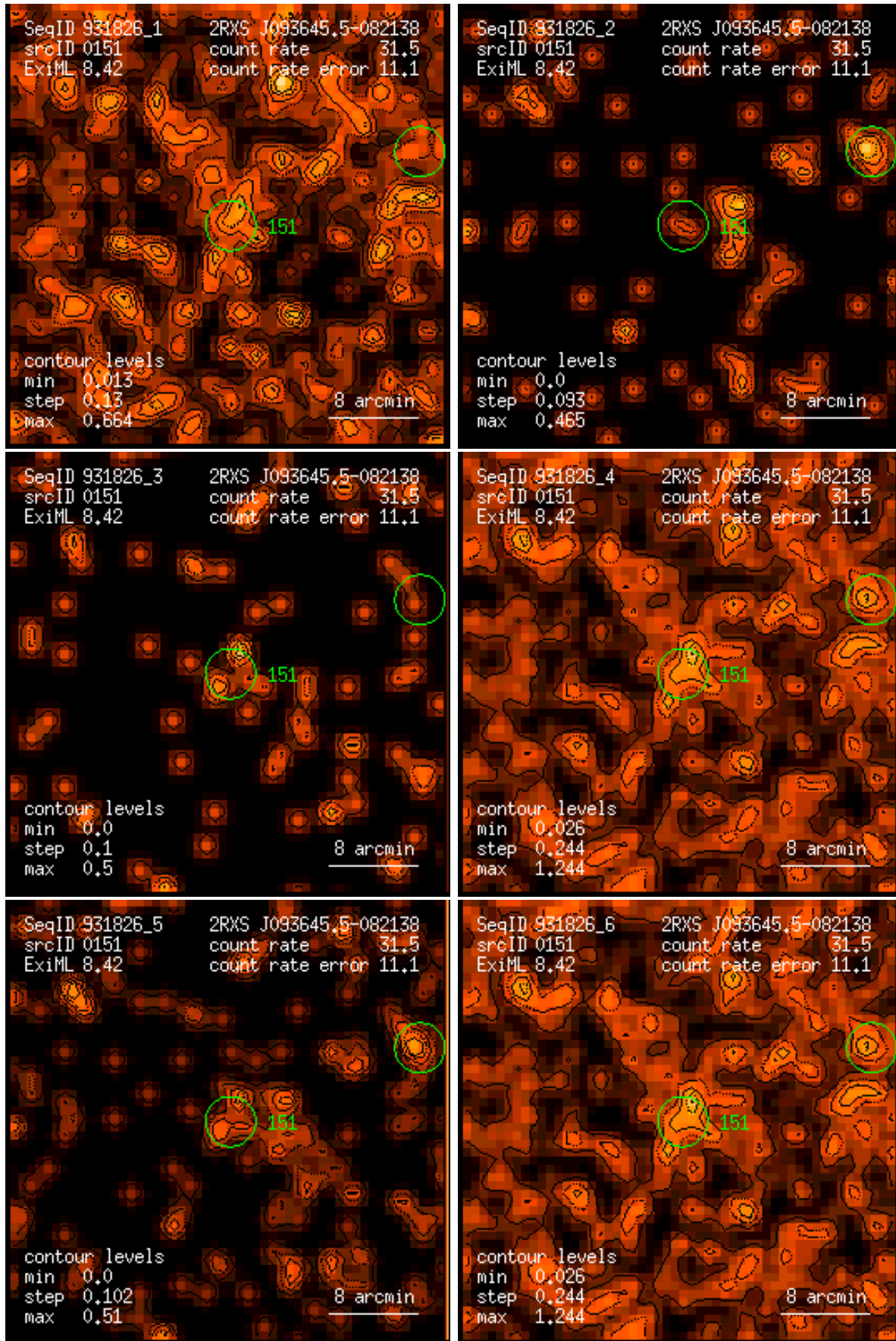
Figure 151: RASS 931826: detection 0151: band rate images, Gaussian filter: (1) PSPC channels 11 – 41, (2) 52 – 90, (3) 91 – 201, (4) 11 – 235, (5) 52 – 201, (6) 11 – 201. Broad band rates in counts/ks. Band rate contour levels in counts/ks/arcmin 2 .
