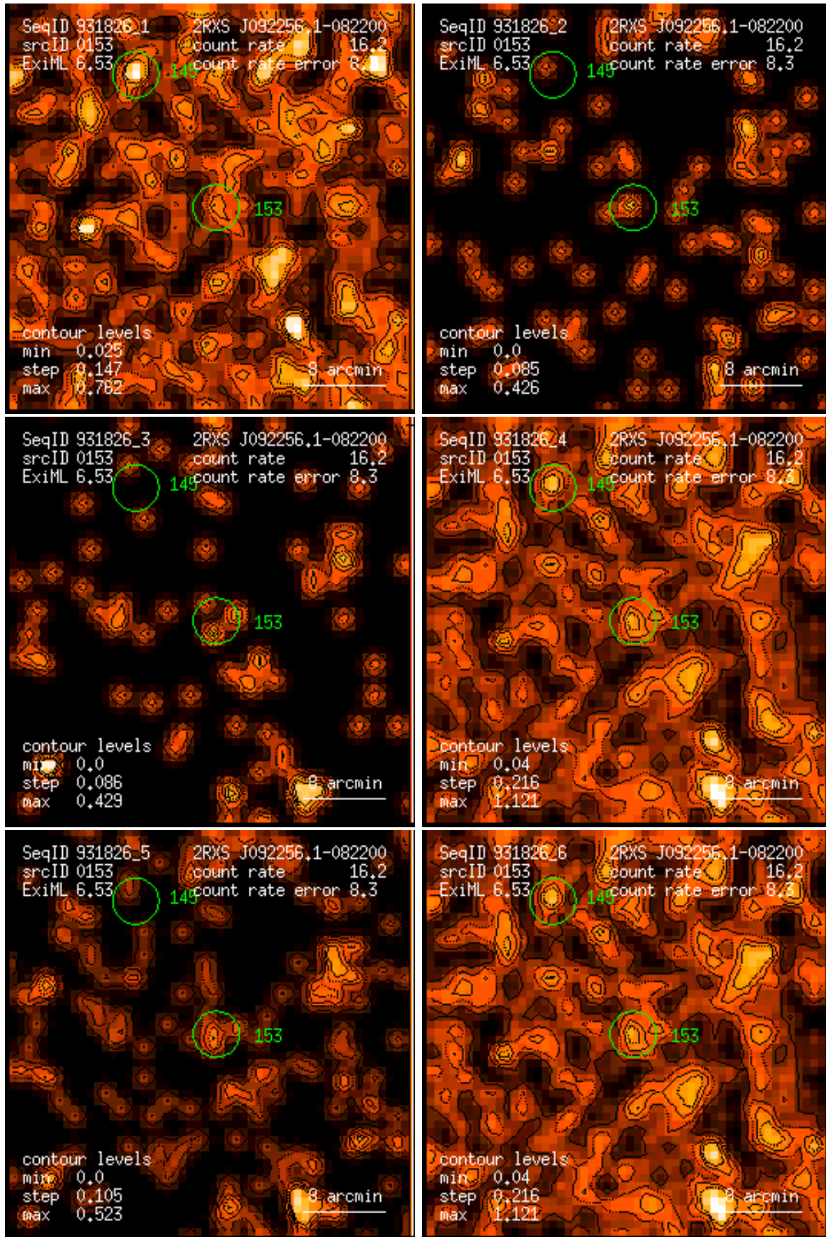
Figure 153: RASS 931826: detection 0153: band rate images, Gaussian filter: (1) PSPC channels 11 – 41, (2) 52 – 90, (3) 91 – 201, (4) 11 – 235, (5) 52 – 201, (6) 11 – 201. Broad band rates in counts/ks. Band rate contour levels in counts/ks/arcmin 2 .
