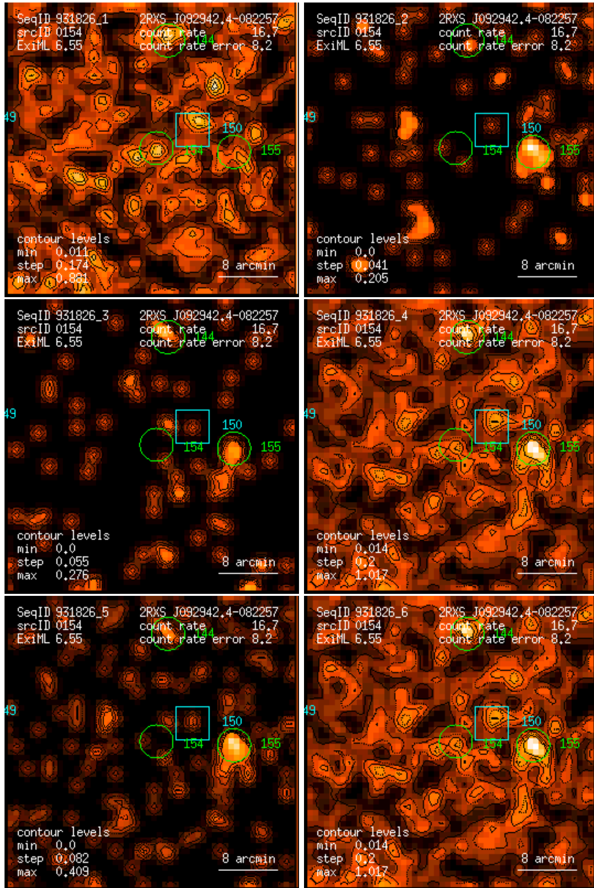
Figure 154: RASS 931826: detection 0154: band rate images, Gaussian filter: (1) PSPC channels 11 – 41, (2) 52 – 90, (3) 91 – 201, (4) 11 – 235, (5) 52 – 201, (6) 11 – 201. Broad band rates in counts/ks. Band rate contour levels in counts/ks/arcmin 2 .
