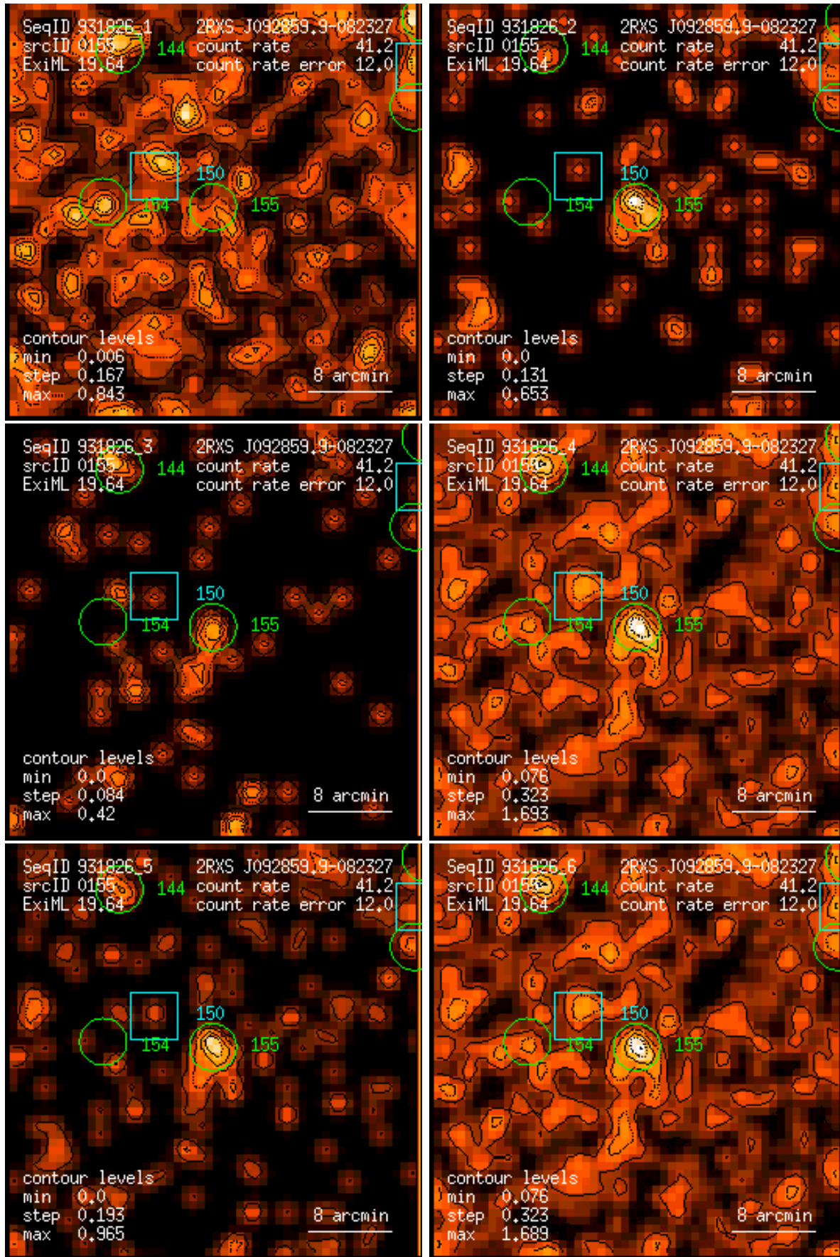
Figure 155: RASS 931826: detection 0155: band rate images, Gaussian filter: (1) PSPC channels 11 – 41, (2) 52 – 90, (3) 91 – 201, (4) 11 – 235, (5) 52 – 201, (6) 11 – 201. Broad band rates in counts/ks. Band rate contour levels in counts/ks/arcmin 2 .
