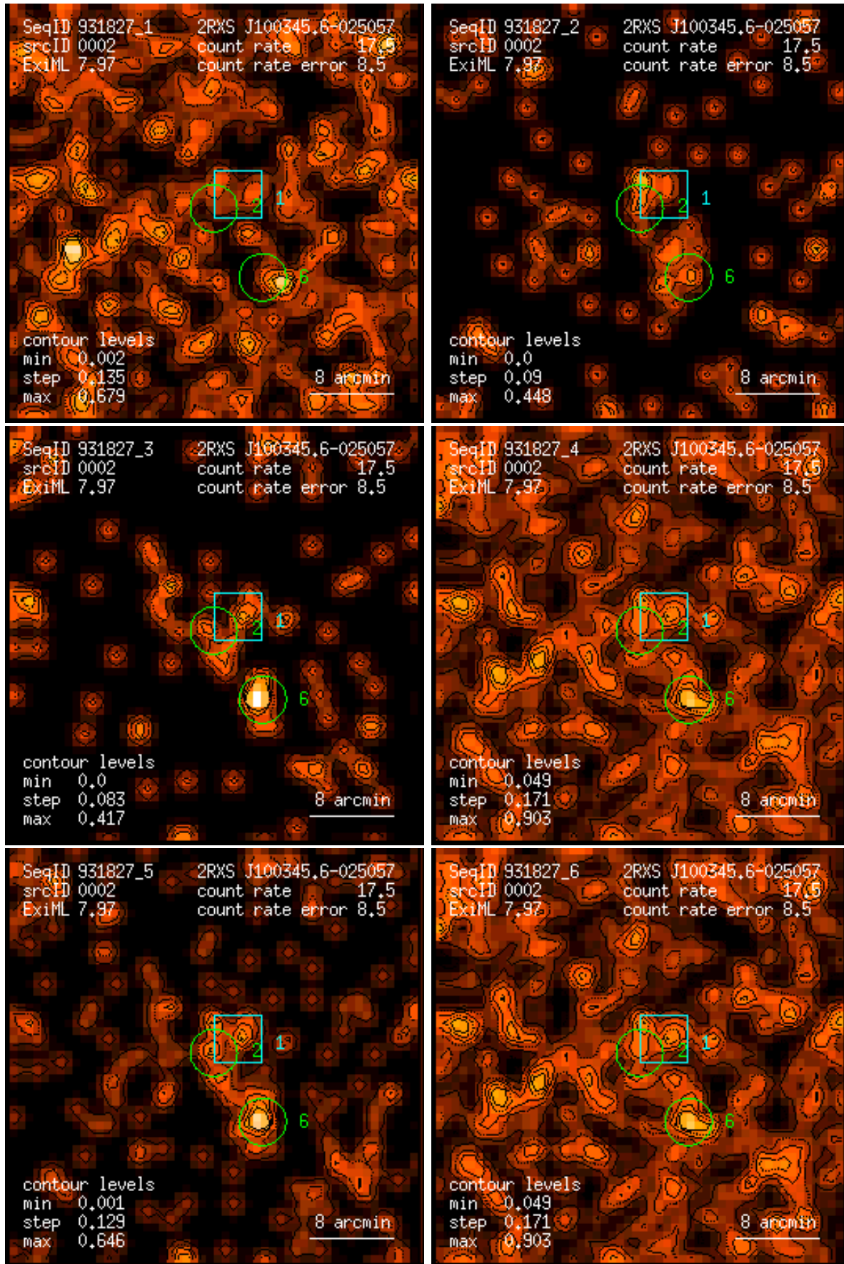
Figure 2: RASS 931827: detection 0002: band rate images, Gaussian filter: (1) PSPC channels 11 – 41, (2) 52 – 90, (3) 91 – 201, (4) 11 – 235, (5) 52 – 201, (6) 11 – 201. Broad band rates in counts/ks. Band rate contour levels in counts/ks/arcmin 2 .
