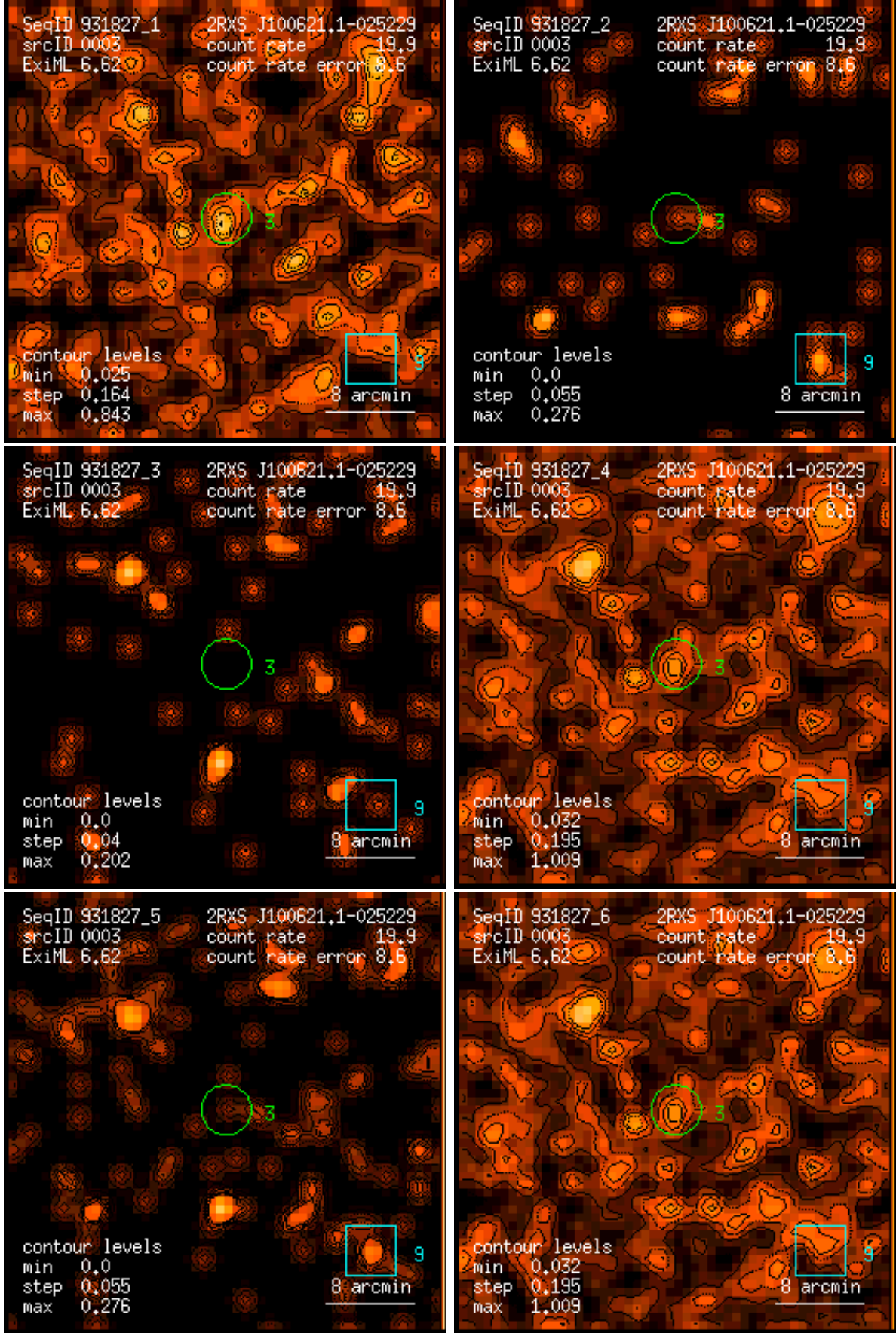
Figure 3: RASS 931827: detection 0003: band rate images, Gaussian filter: (1) PSPC channels 11 – 41, (2) 52 – 90, (3) 91 – 201, (4) 11 – 235, (5) 52 – 201, (6) 11 – 201. Broad band rates in counts/ks. Band rate contour levels in counts/ks/arcmin 2 .
