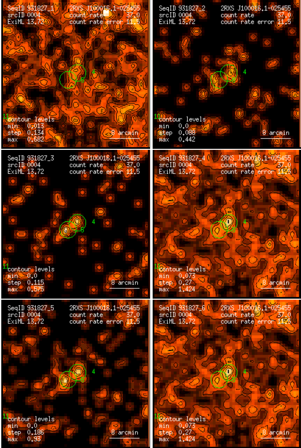
Figure 4: RASS 931827: detection 0004: band rate images, Gaussian filter: (1) PSPC channels 11 – 41, (2) 52 – 90, (3) 91 – 201, (4) 11 – 235, (5) 52 – 201, (6) 11 – 201. Broad band rates in counts/ks. Band rate contour levels in counts/ks/arcmin 2 .
