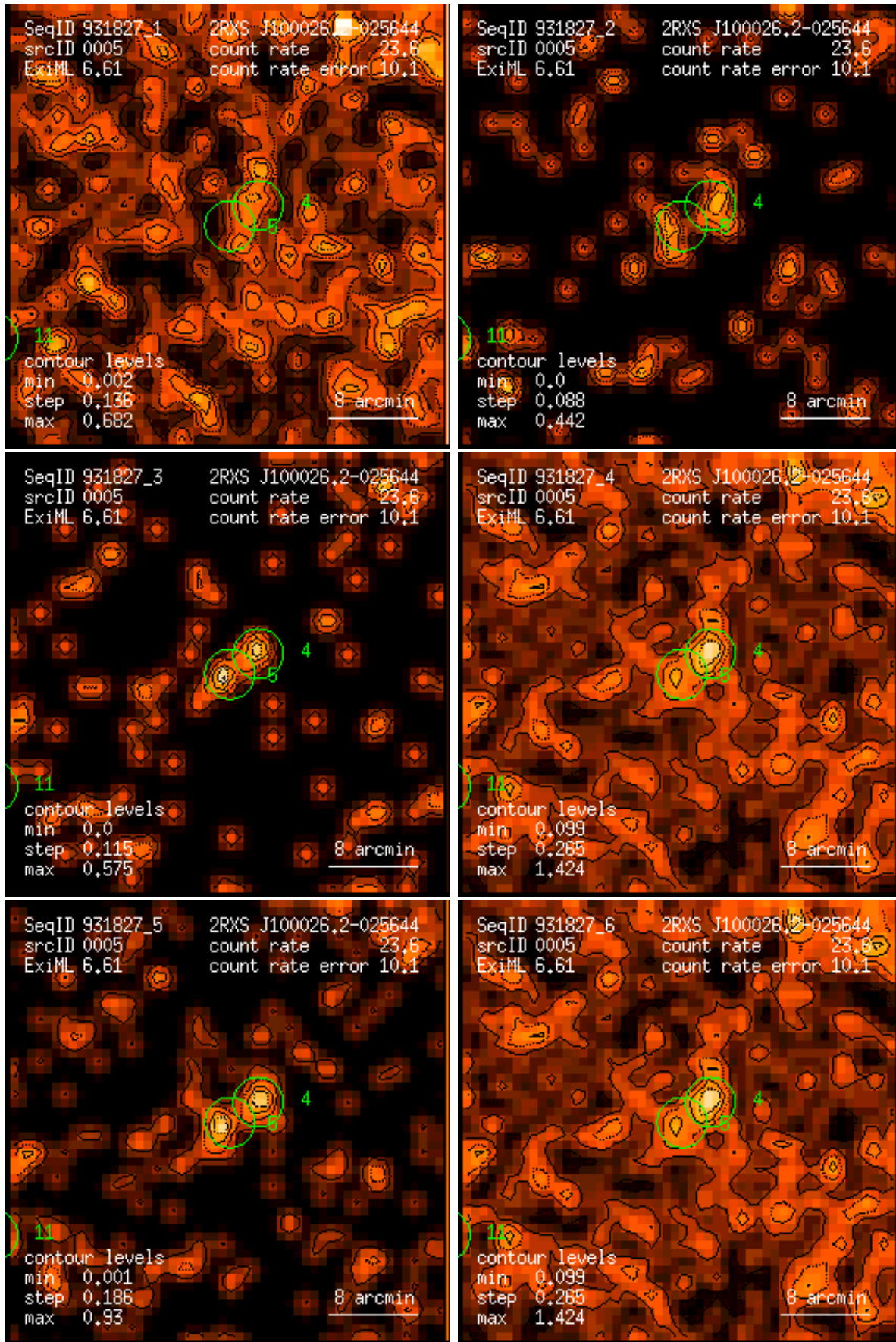
Figure 5: RASS 931827: detection 0005: band rate images, Gaussian filter: (1) PSPC channels 11 – 41, (2) 52 – 90, (3) 91 – 201, (4) 11 – 235, (5) 52 – 201, (6) 11 – 201. Broad band rates in counts/ks. Band rate contour levels in counts/ks/arcmin 2 .
