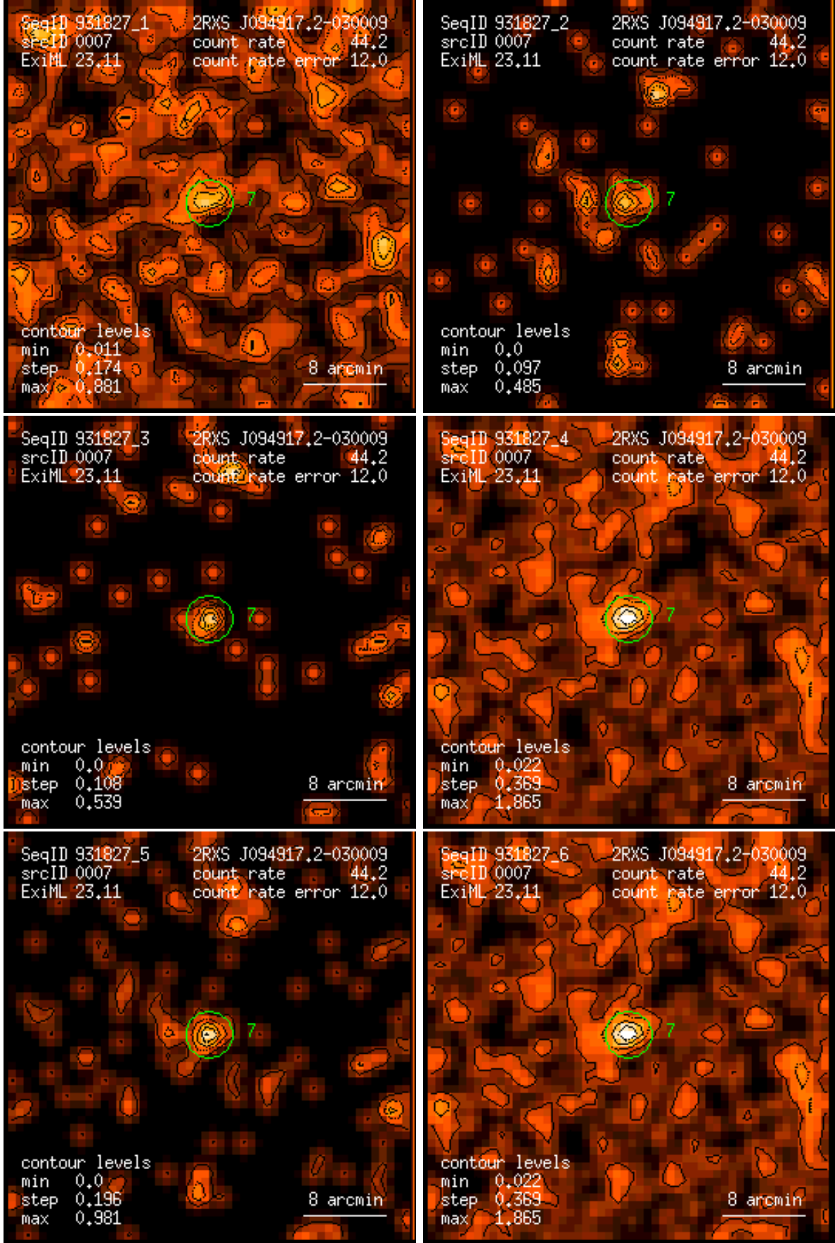
Figure 7: RASS 931827: detection 0007: band rate images, Gaussian filter: (1) PSPC channels 11 – 41, (2) 52 – 90, (3) 91 – 201, (4) 11 – 235, (5) 52 – 201, (6) 11 – 201. Broad band rates in counts/ks. Band rate contour levels in counts/ks/arcmin 2 .
