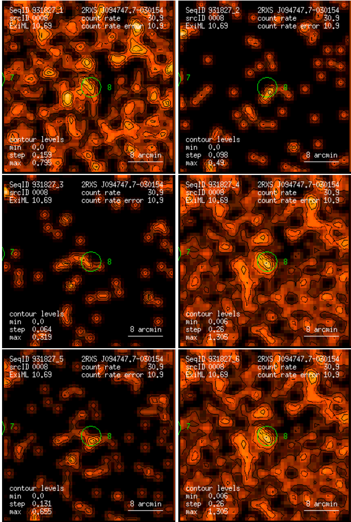
Figure 8: RASS 931827: detection 0008: band rate images, Gaussian filter: (1) PSPC channels 11 – 41, (2) 52 – 90, (3) 91 – 201, (4) 11 – 235, (5) 52 – 201, (6) 11 – 201. Broad band rates in counts/ks. Band rate contour levels in counts/ks/arcmin 2 .
