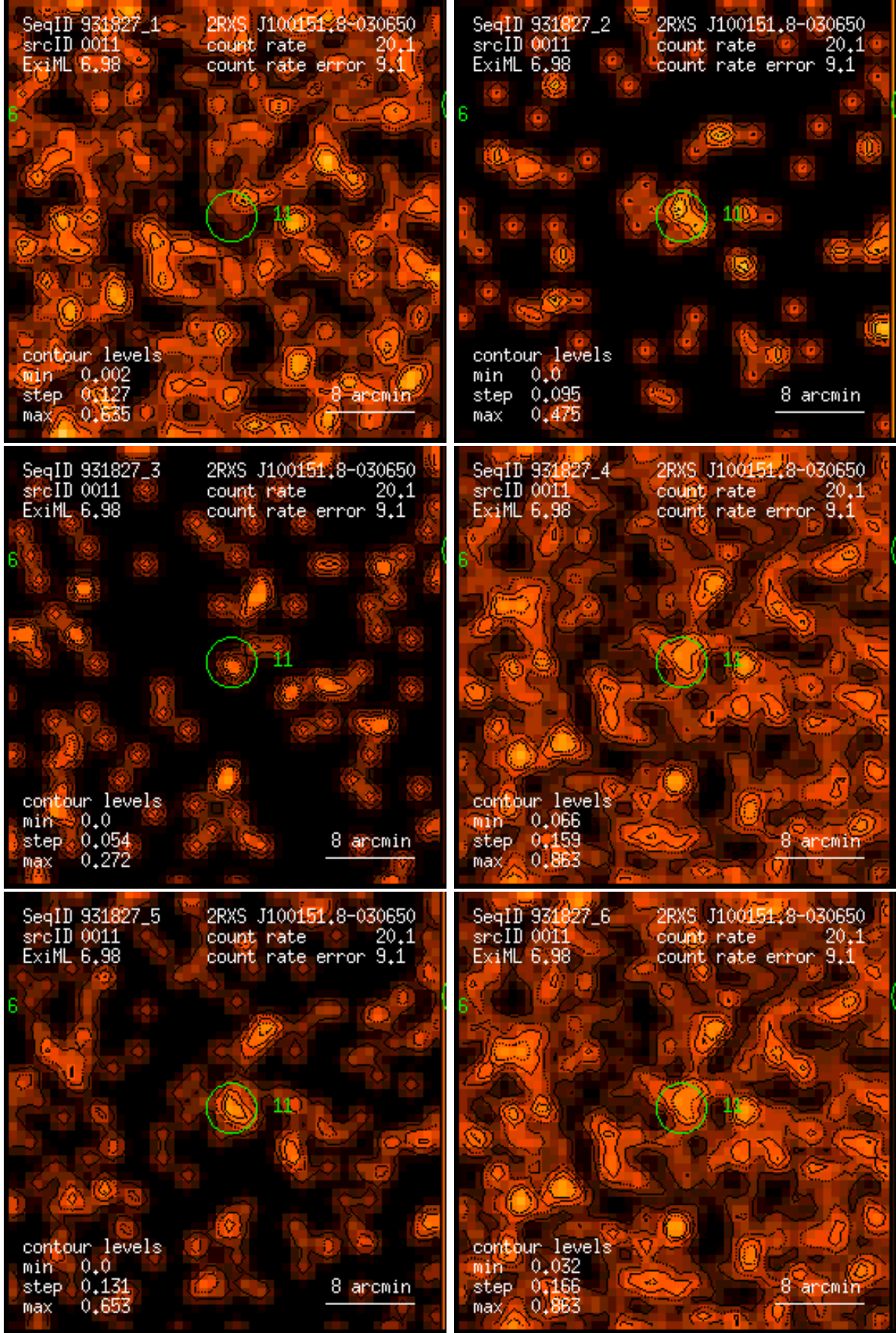
Figure 11: RASS 931827: detection 0011: band rate images, Gaussian filter: (1) PSPC channels 11 – 41, (2) 52 – 90, (3) 91 – 201, (4) 11 – 235, (5) 52 – 201, (6) 11 – 201. Broad band rates in counts/ks. Band rate contour levels in counts/ks/arcmin 2 .
