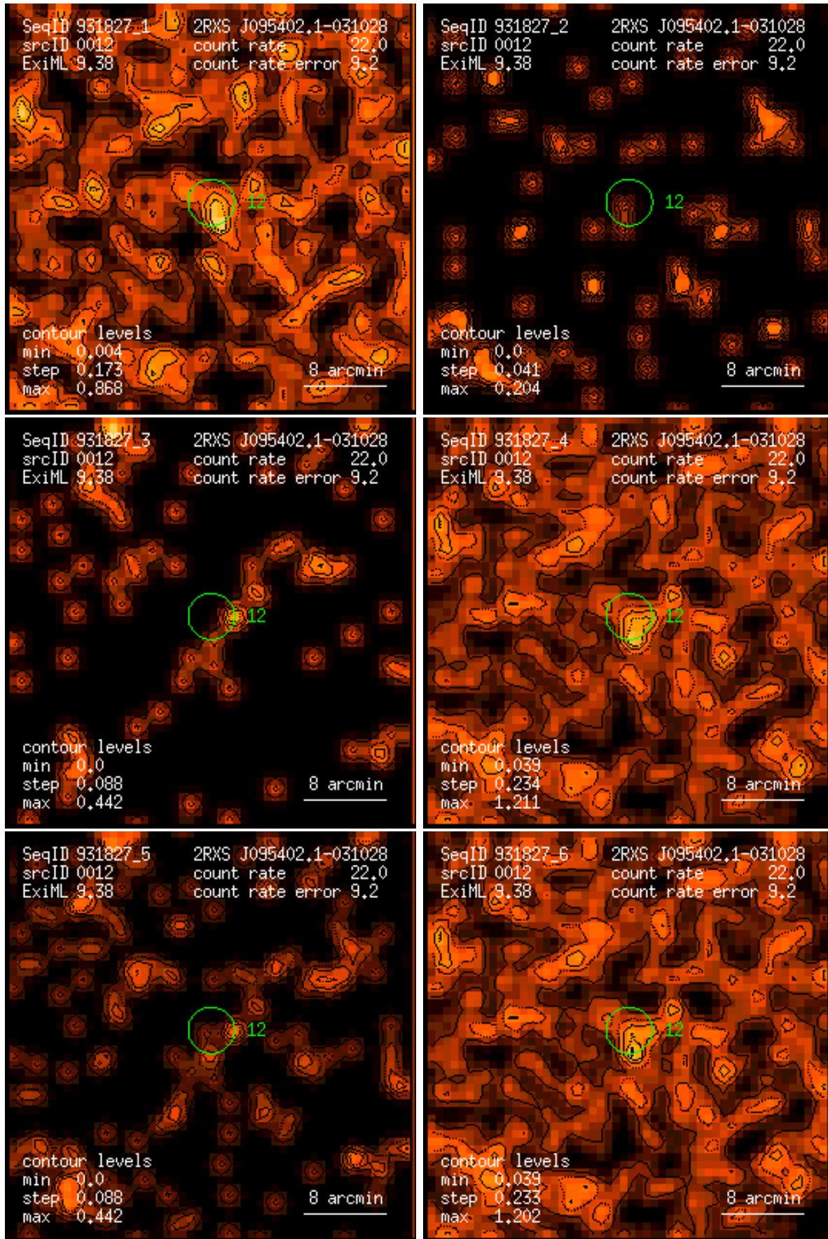
Figure 12: RASS 931827: detection 0012: band rate images, Gaussian filter: (1) PSPC channels 11 – 41, (2) 52 – 90, (3) 91 – 201, (4) 11 – 235, (5) 52 – 201, (6) 11 – 201. Broad band rates in counts/ks. Band rate contour levels in counts/ks/arcmin 2 .
