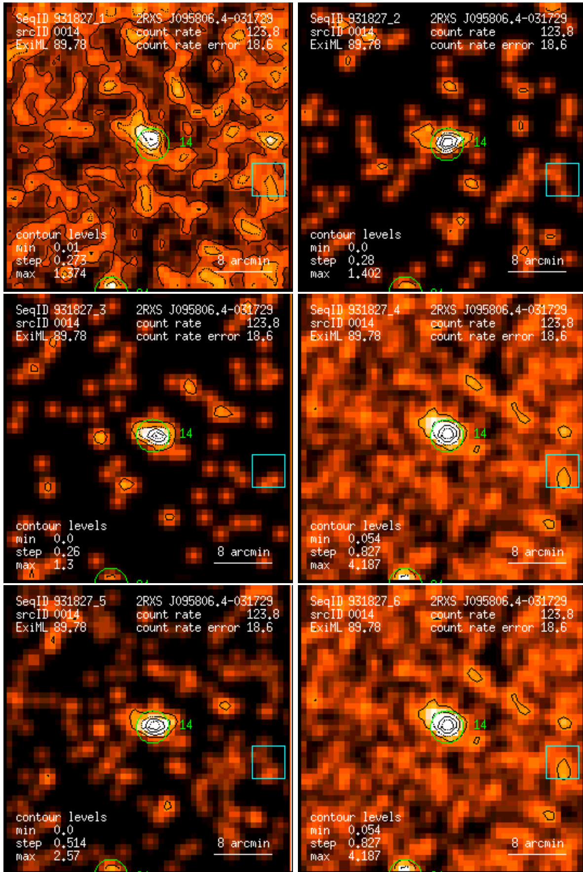
Figure 14: RASS 931827: detection 0014: band rate images, Gaussian filter: (1) PSPC channels 11 – 41, (2) 52 – 90, (3) 91 – 201, (4) 11 – 235, (5) 52 – 201, (6) 11 – 201. Broad band rates in counts/ks. Band rate contour levels in counts/ks/arcmin 2 .
