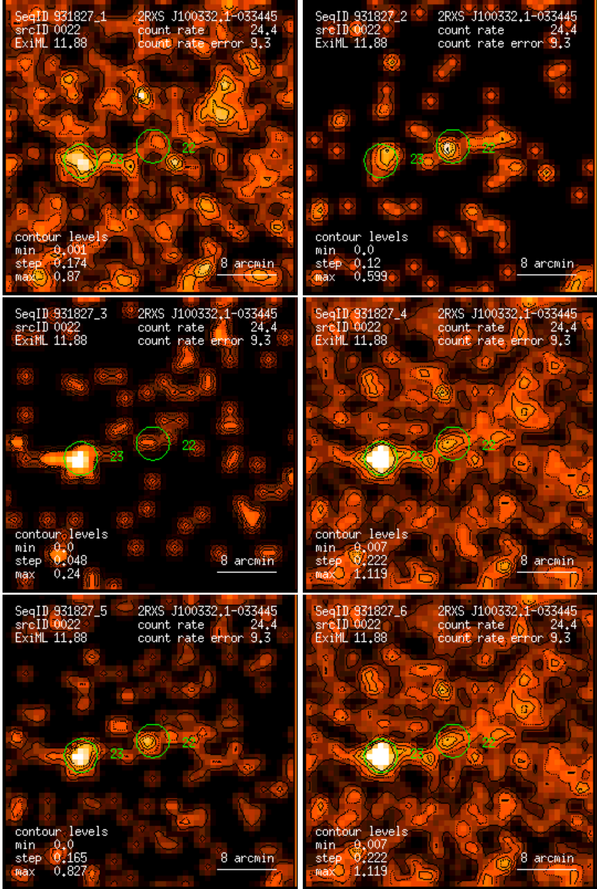
Figure 22: RASS 931827: detection 0022: band rate images, Gaussian filter: (1) PSPC channels 11 – 41, (2) 52 – 90, (3) 91 – 201, (4) 11 – 235, (5) 52 – 201, (6) 11 – 201. Broad band rates in counts/ks. Band rate contour levels in counts/ks/arcmin 2 .
