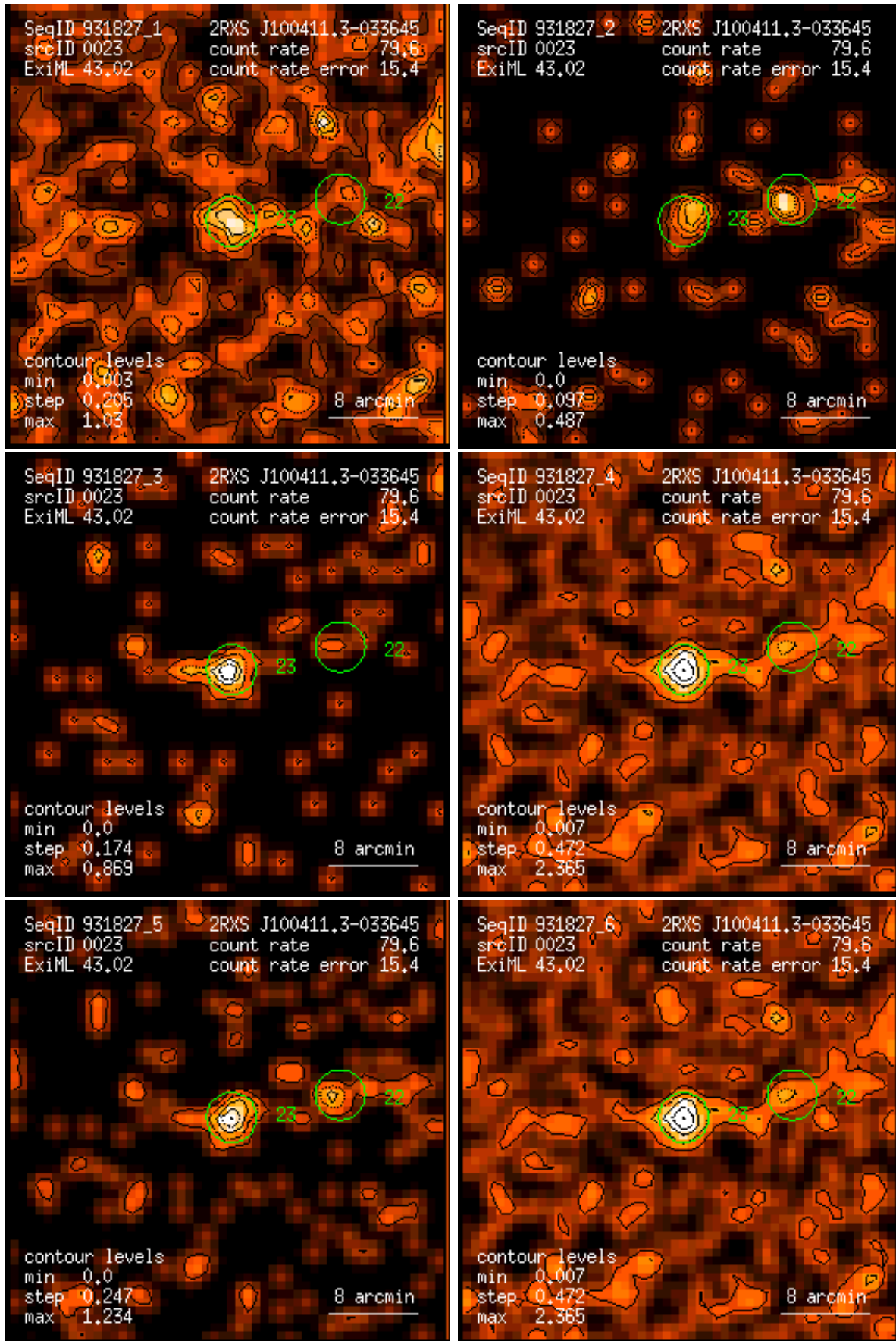
Figure 23: RASS 931827: detection 0023: band rate images, Gaussian filter: (1) PSPC channels 11 – 41, (2) 52 – 90, (3) 91 – 201, (4) 11 – 235, (5) 52 – 201, (6) 11 – 201. Broad band rates in counts/ks. Band rate contour levels in counts/ks/arcmin 2 .
