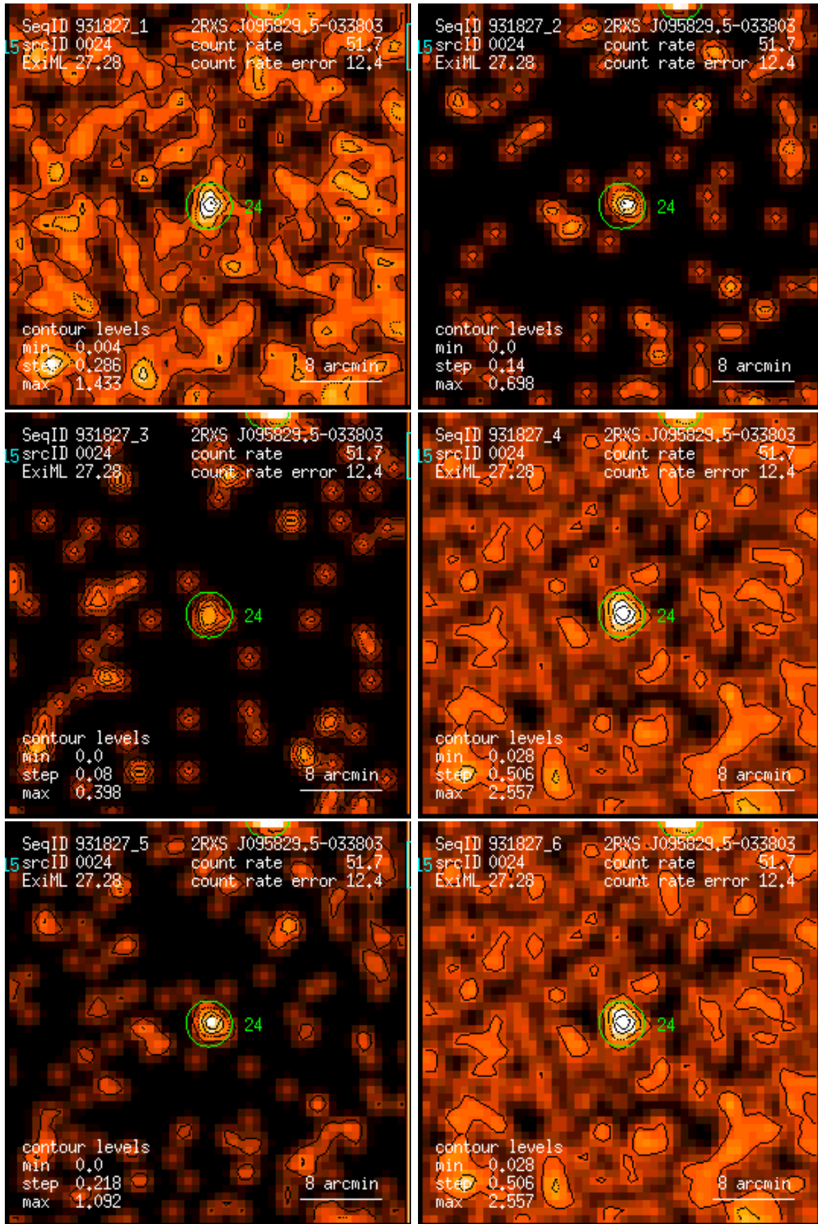
Figure 24: RASS 931827: detection 0024: band rate images, Gaussian filter: (1) PSPC channels 11 – 41, (2) 52 – 90, (3) 91 – 201, (4) 11 – 235, (5) 52 – 201, (6) 11 – 201. Broad band rates in counts/ks. Band rate contour levels in counts/ks/arcmin 2 .
