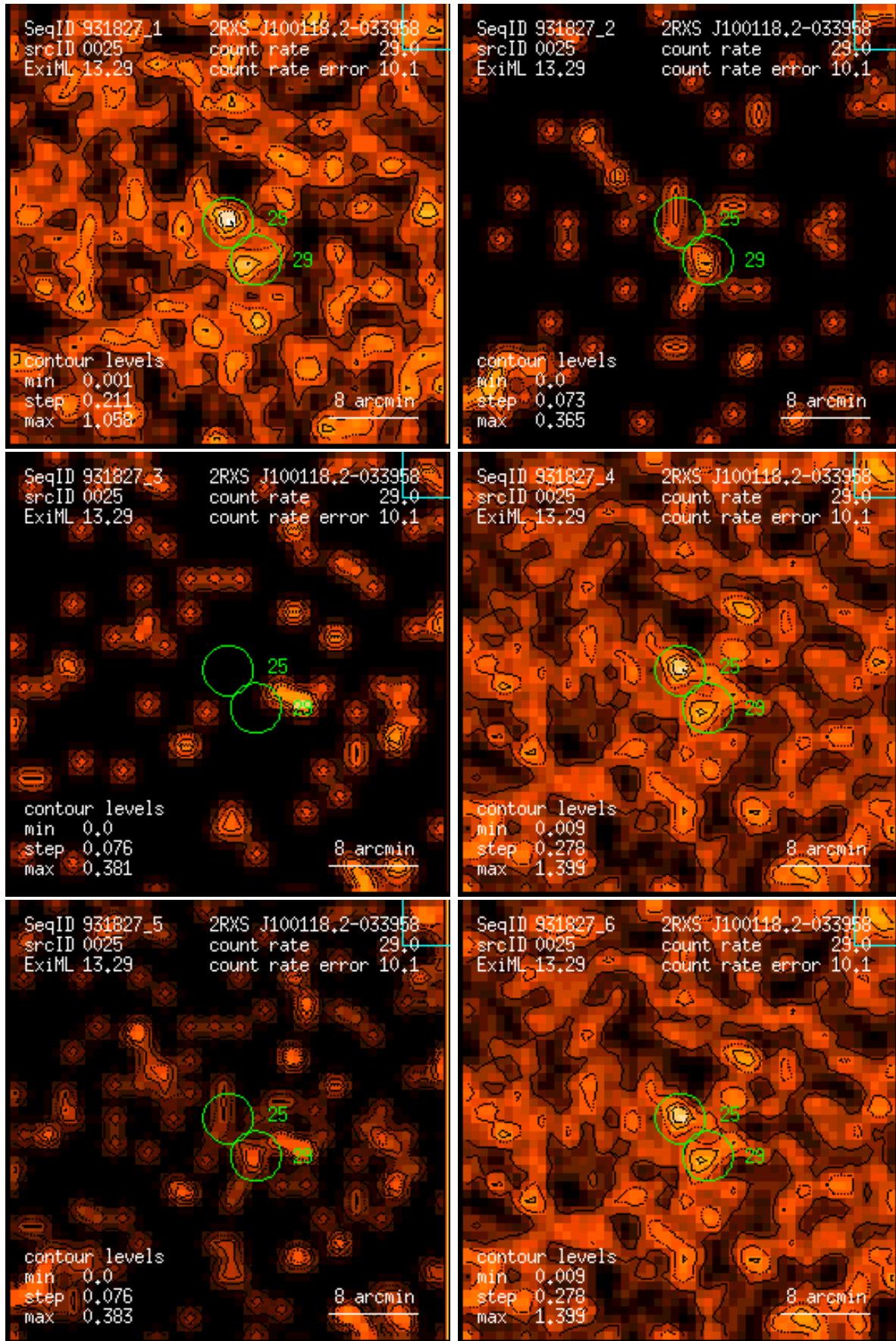
Figure 25: RASS 931827: detection 0025: band rate images, Gaussian filter: (1) PSPC channels 11 – 41, (2) 52 – 90, (3) 91 – 201, (4) 11 – 235, (5) 52 – 201, (6) 11 – 201. Broad band rates in counts/ks. Band rate contour levels in counts/ks/arcmin 2 .
