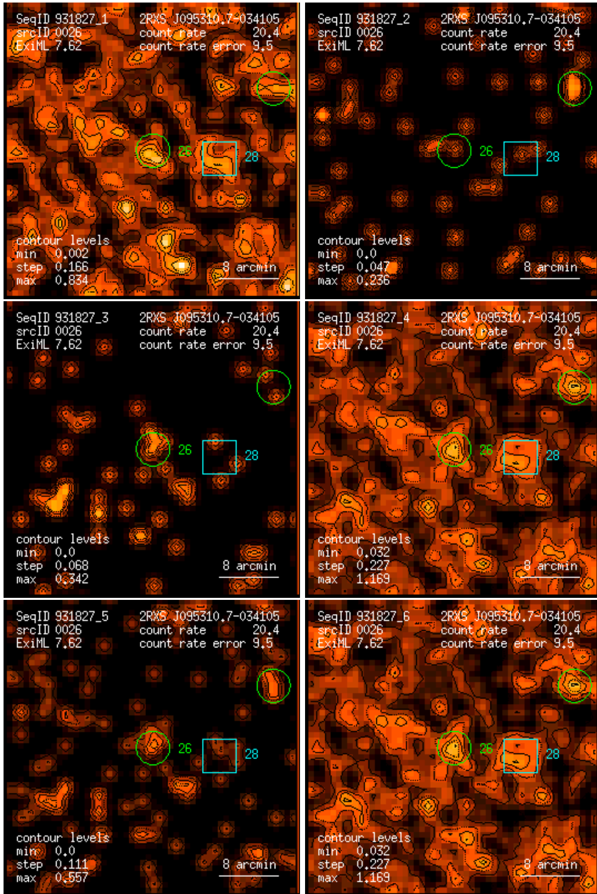
Figure 26: RASS 931827: detection 0026: band rate images, Gaussian filter: (1) PSPC channels 11 – 41, (2) 52 – 90, (3) 91 – 201, (4) 11 – 235, (5) 52 – 201, (6) 11 – 201. Broad band rates in counts/ks. Band rate contour levels in counts/ks/arcmin 2 .
