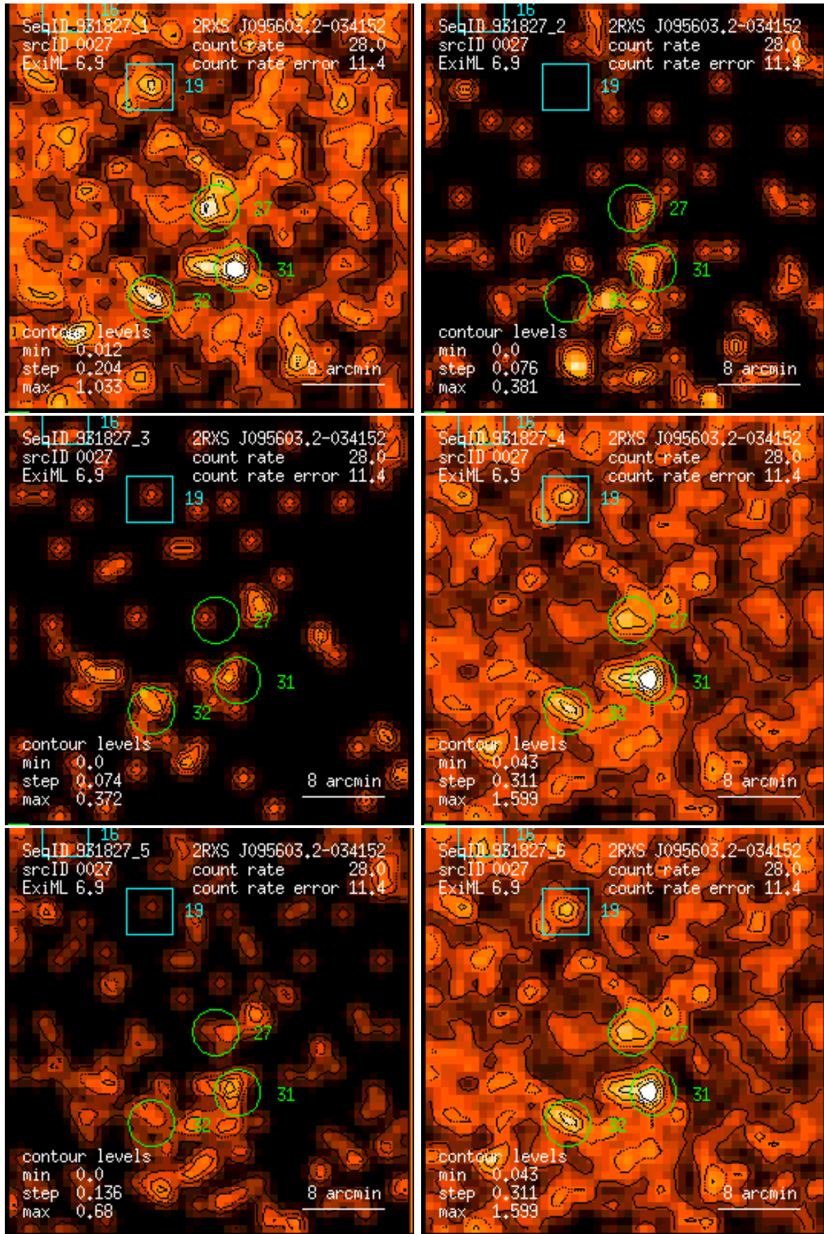
Figure 27: RASS 931827: detection 0027: band rate images, Gaussian filter: (1) PSPC channels 11 – 41, (2) 52 – 90, (3) 91 – 201, (4) 11 – 235, (5) 52 – 201, (6) 11 – 201. Broad band rates in counts/ks. Band rate contour levels in counts/ks/arcmin 2 .
