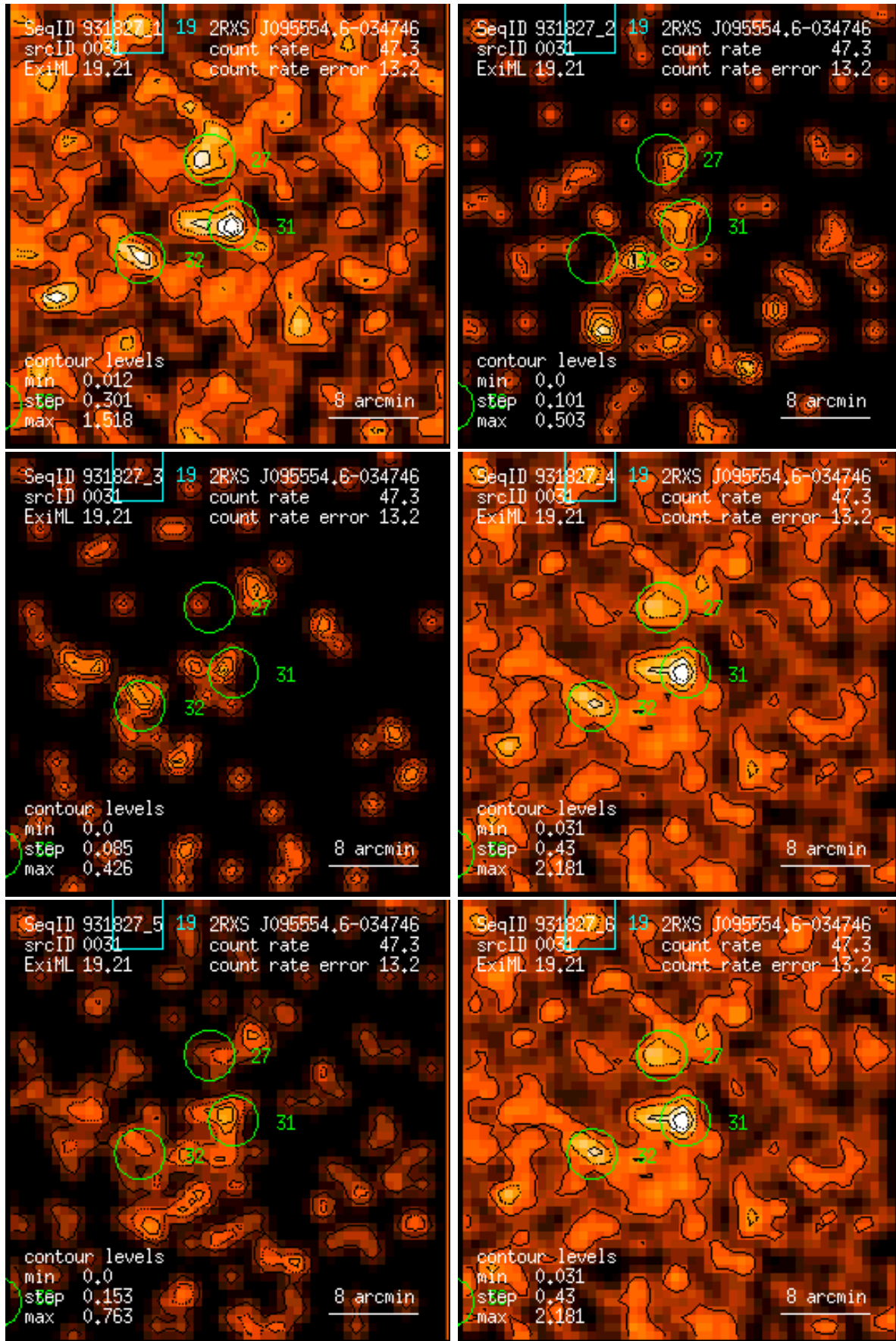
Figure 31: RASS 931827: detection 0031: band rate images, Gaussian filter: (1) PSPC channels 11 – 41, (2) 52 – 90, (3) 91 – 201, (4) 11 – 235, (5) 52 – 201, (6) 11 – 201. Broad band rates in counts/ks. Band rate contour levels in counts/ks/arcmin 2 .
