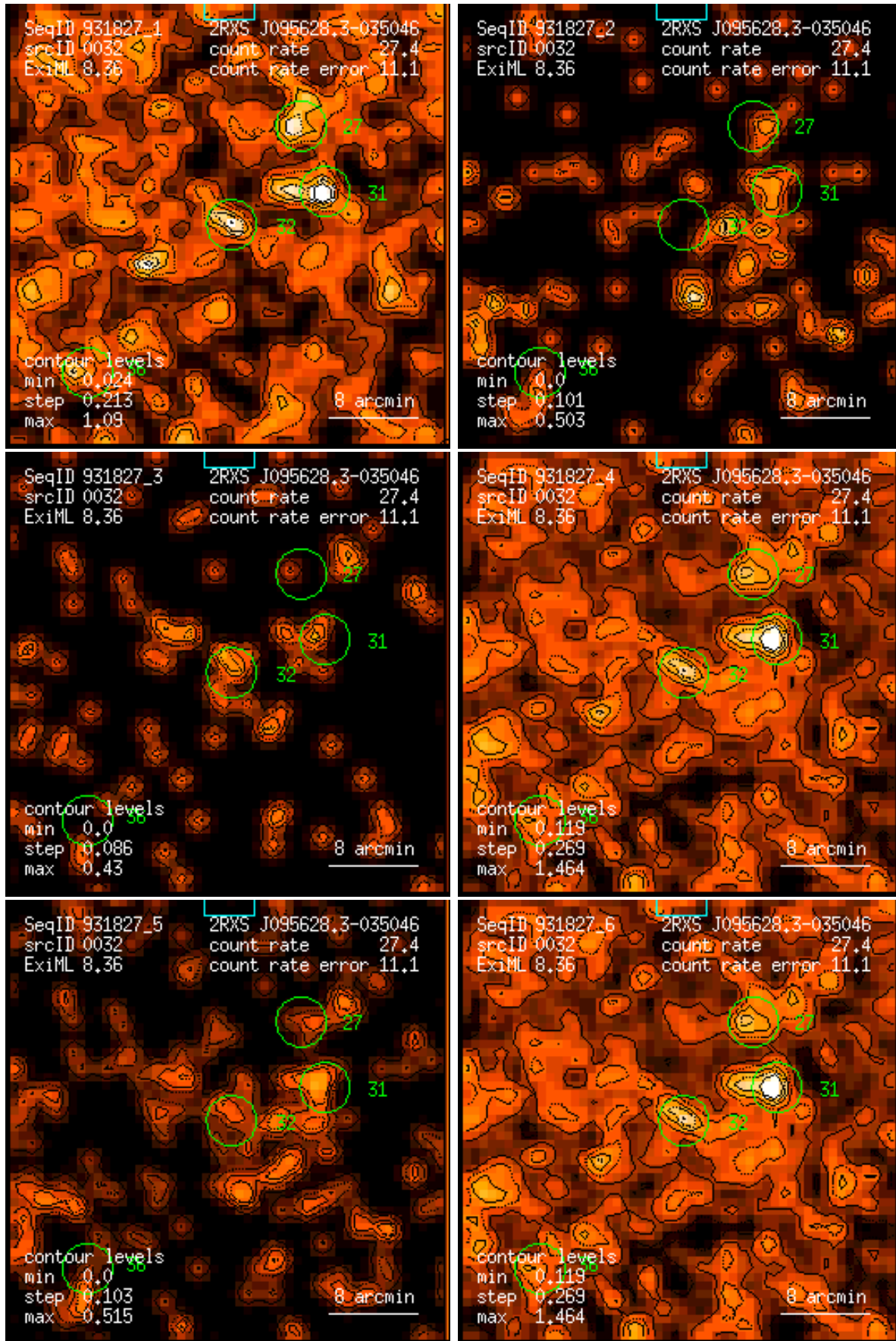
Figure 32: RASS 931827: detection 0032: band rate images, Gaussian filter: (1) PSPC channels 11 – 41, (2) 52 – 90, (3) 91 – 201, (4) 11 – 235, (5) 52 – 201, (6) 11 – 201. Broad band rates in counts/ks. Band rate contour levels in counts/ks/arcmin 2 .
