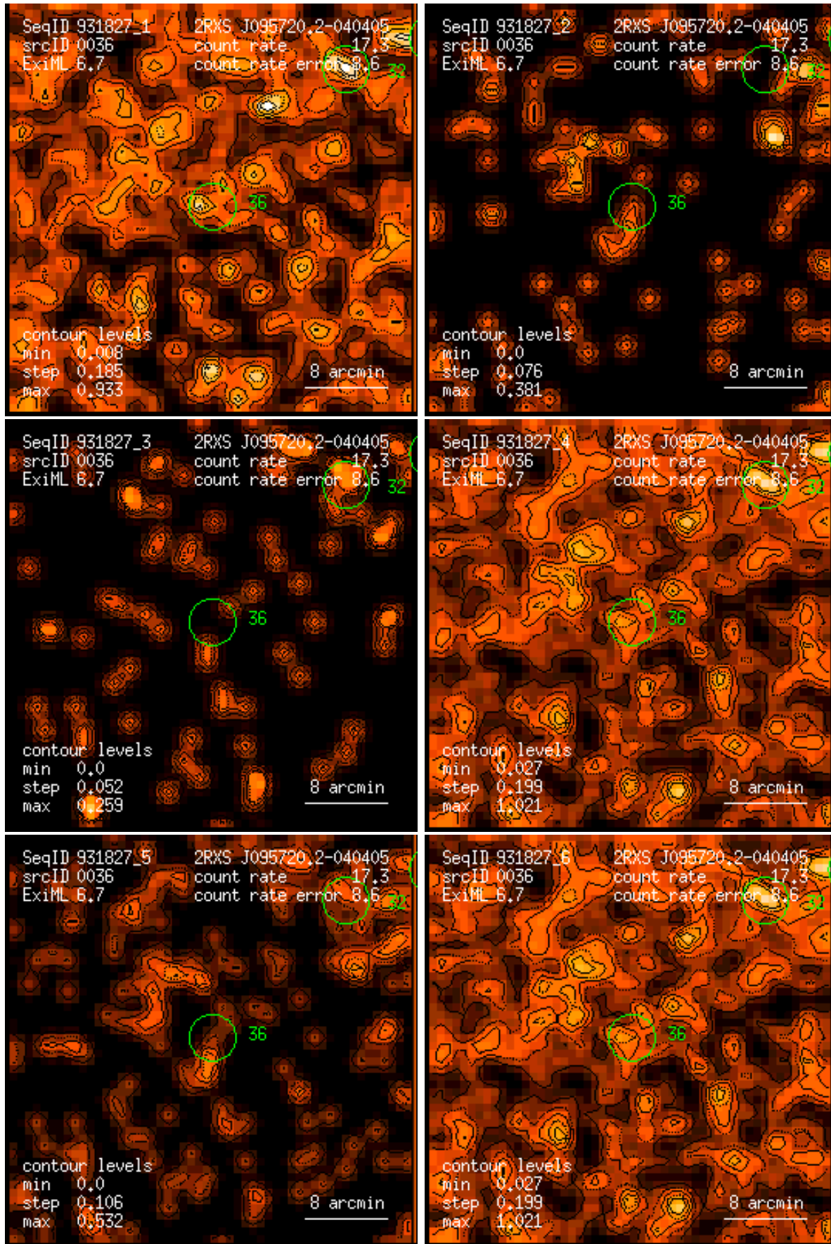
Figure 36: RASS 931827: detection 0036: band rate images, Gaussian filter: (1) PSPC channels 11 – 41, (2) 52 – 90, (3) 91 – 201, (4) 11 – 235, (5) 52 – 201, (6) 11 – 201. Broad band rates in counts/ks. Band rate contour levels in counts/ks/arcmin 2 .
