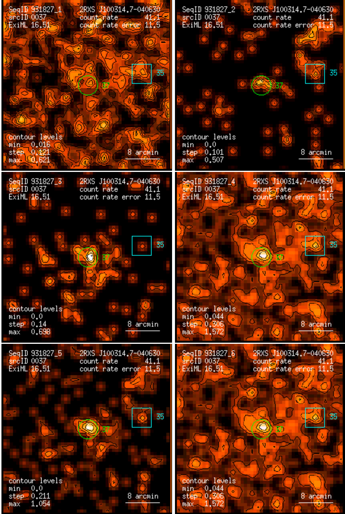
Figure 37: RASS 931827: detection 0037: band rate images, Gaussian filter: (1) PSPC channels 11 – 41, (2) 52 – 90, (3) 91 – 201, (4) 11 – 235, (5) 52 – 201, (6) 11 – 201. Broad band rates in counts/ks. Band rate contour levels in counts/ks/arcmin 2 .
