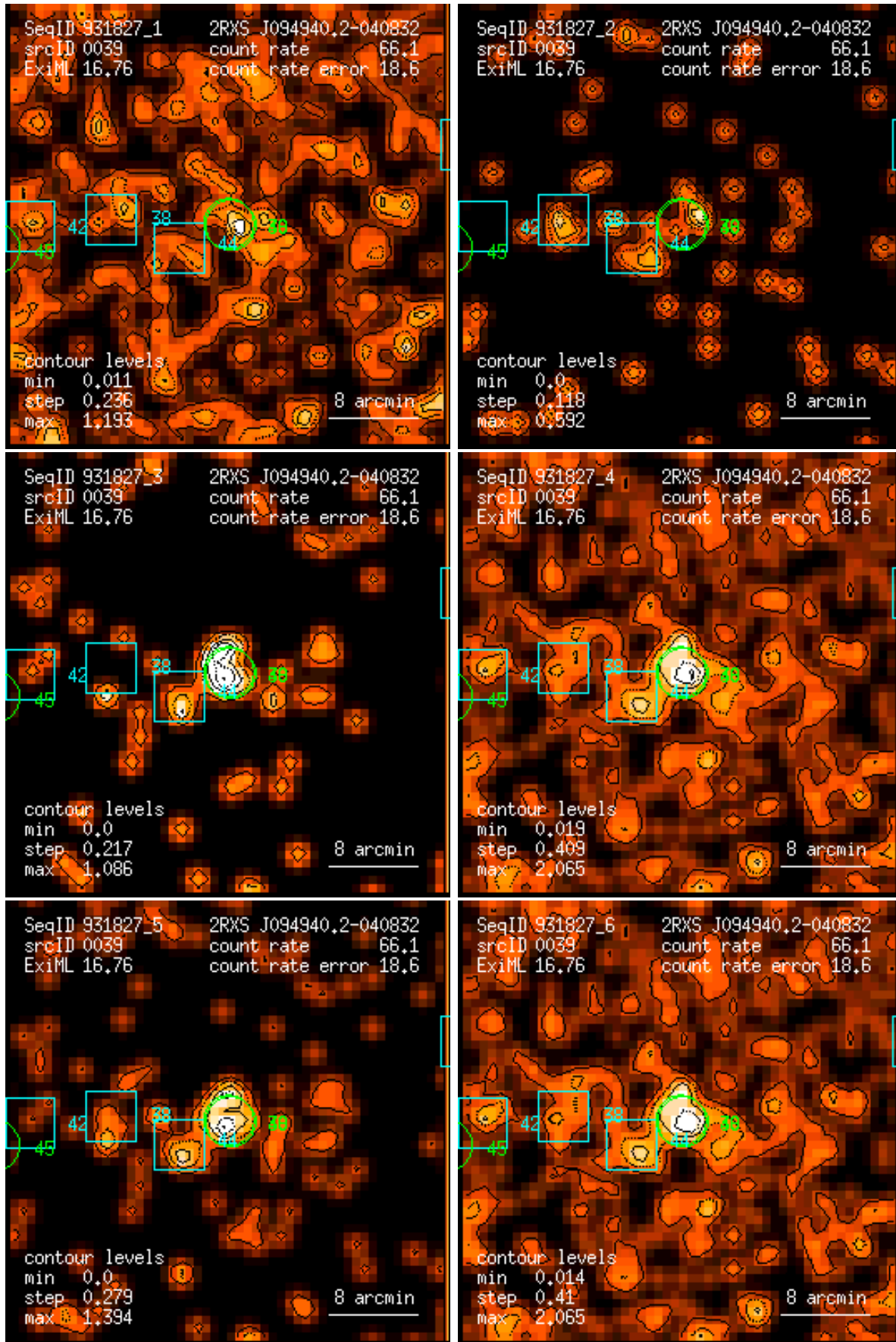
Figure 39: RASS 931827: detection 0039: band rate images, Gaussian filter: (1) PSPC channels 11 – 41, (2) 52 – 90, (3) 91 – 201, (4) 11 – 235, (5) 52 – 201, (6) 11 – 201. Broad band rates in counts/ks. Band rate contour levels in counts/ks/arcmin 2 .
