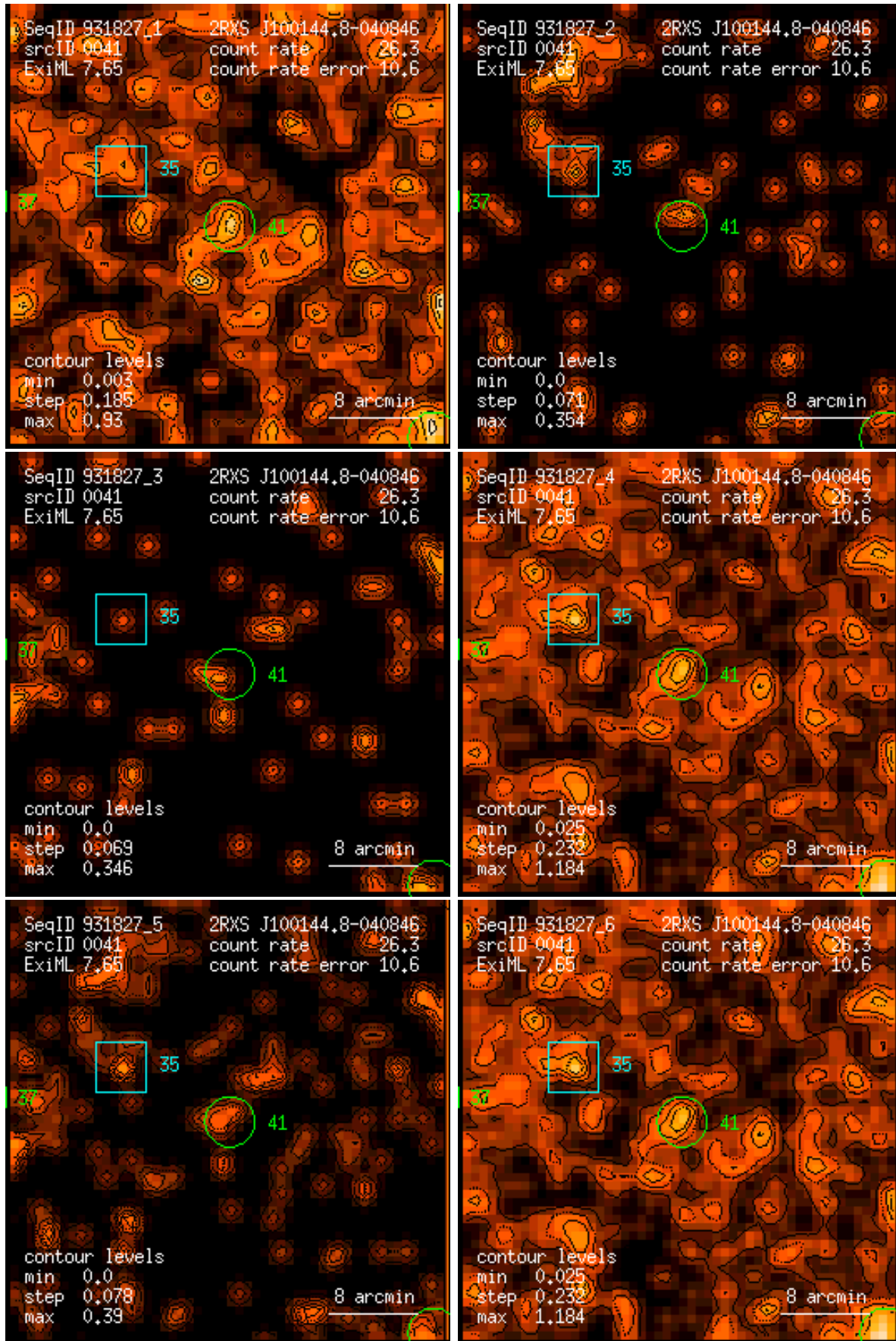
Figure 41: RASS 931827: detection 0041: band rate images, Gaussian filter: (1) PSPC channels 11 – 41, (2) 52 – 90, (3) 91 – 201, (4) 11 – 235, (5) 52 – 201, (6) 11 – 201. Broad band rates in counts/ks. Band rate contour levels in counts/ks/arcmin 2 .
