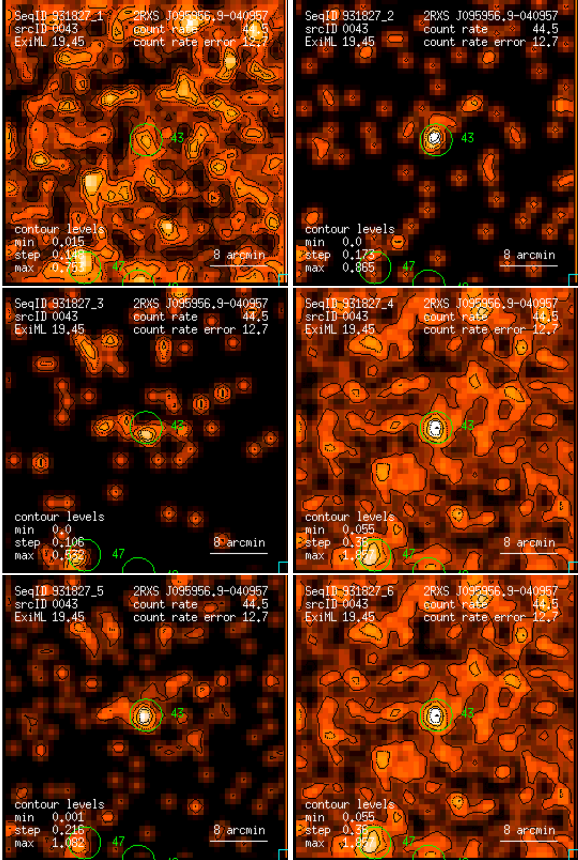
Figure 43: RASS 931827: detection 0043: band rate images, Gaussian filter: (1) PSPC channels 11 – 41, (2) 52 – 90, (3) 91 – 201, (4) 11 – 235, (5) 52 – 201, (6) 11 – 201. Broad band rates in counts/ks. Band rate contour levels in counts/ks/arcmin 2 .
