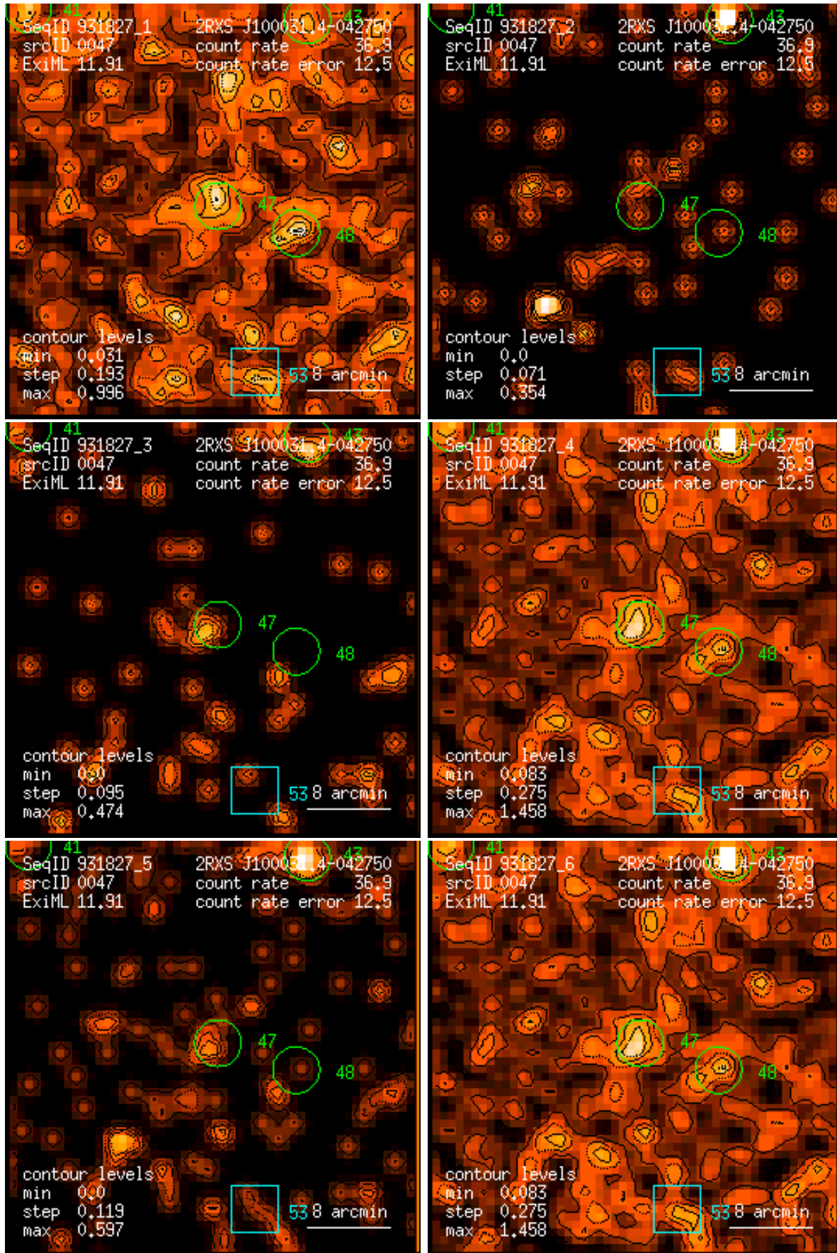
Figure 47: RASS 931827: detection 0047: band rate images, Gaussian filter: (1) PSPC channels 11 – 41, (2) 52 – 90, (3) 91 – 201, (4) 11 – 235, (5) 52 – 201, (6) 11 – 201. Broad band rates in counts/ks. Band rate contour levels in counts/ks/arcmin 2 .
