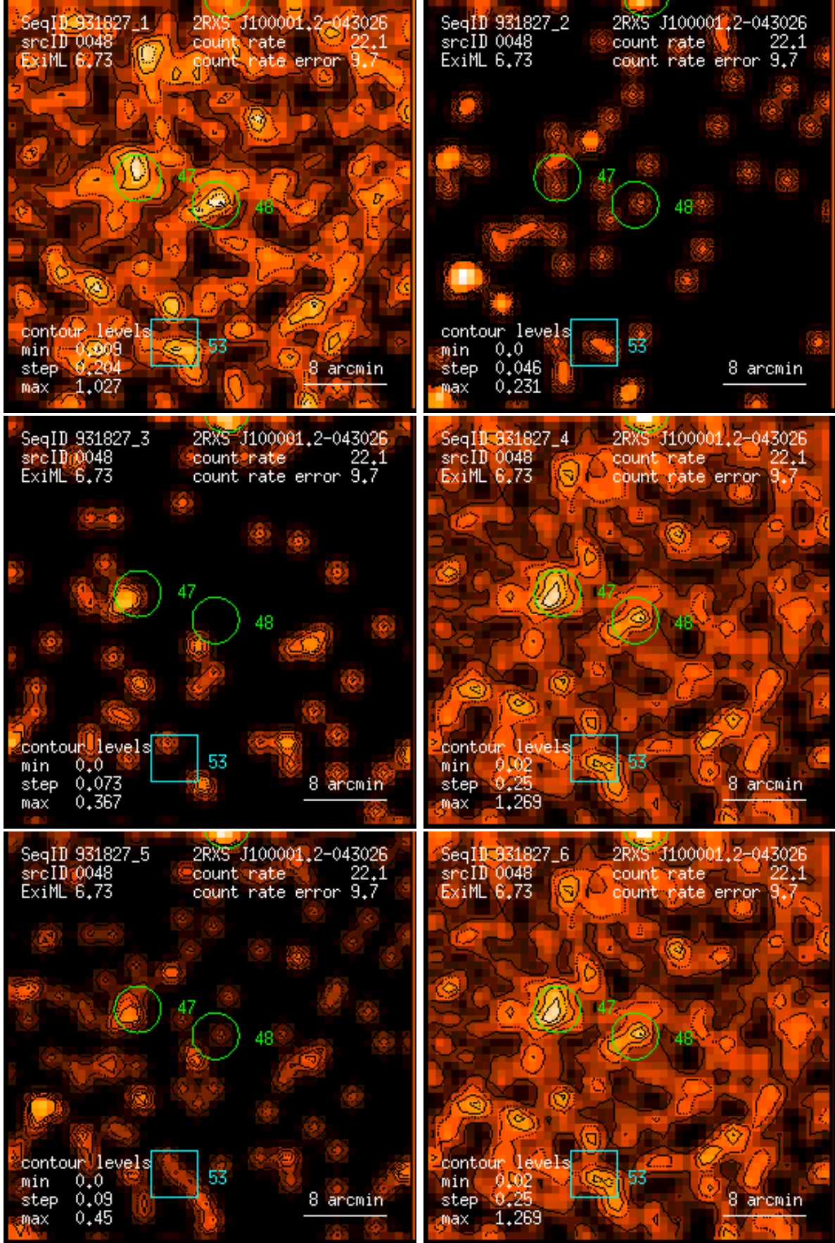
Figure 48: RASS 931827: detection 0048: band rate images, Gaussian filter: (1) PSPC channels 11 – 41, (2) 52 – 90, (3) 91 – 201, (4) 11 – 235, (5) 52 – 201, (6) 11 – 201. Broad band rates in counts/ks. Band rate contour levels in counts/ks/arcmin 2 .
