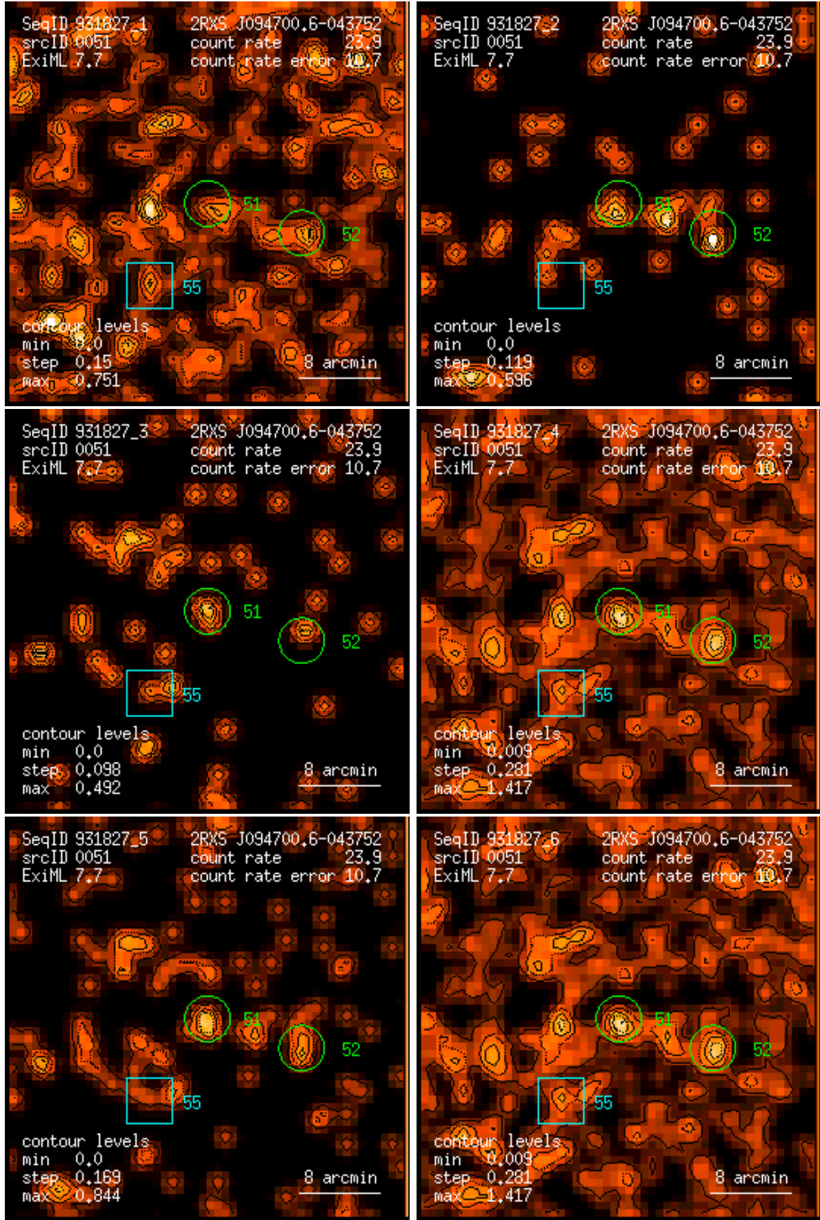
Figure 51: RASS 931827: detection 0051: band rate images, Gaussian filter: (1) PSPC channels 11 – 41, (2) 52 – 90, (3) 91 – 201, (4) 11 – 235, (5) 52 – 201, (6) 11 – 201. Broad band rates in counts/ks. Band rate contour levels in counts/ks/arcmin 2 .
