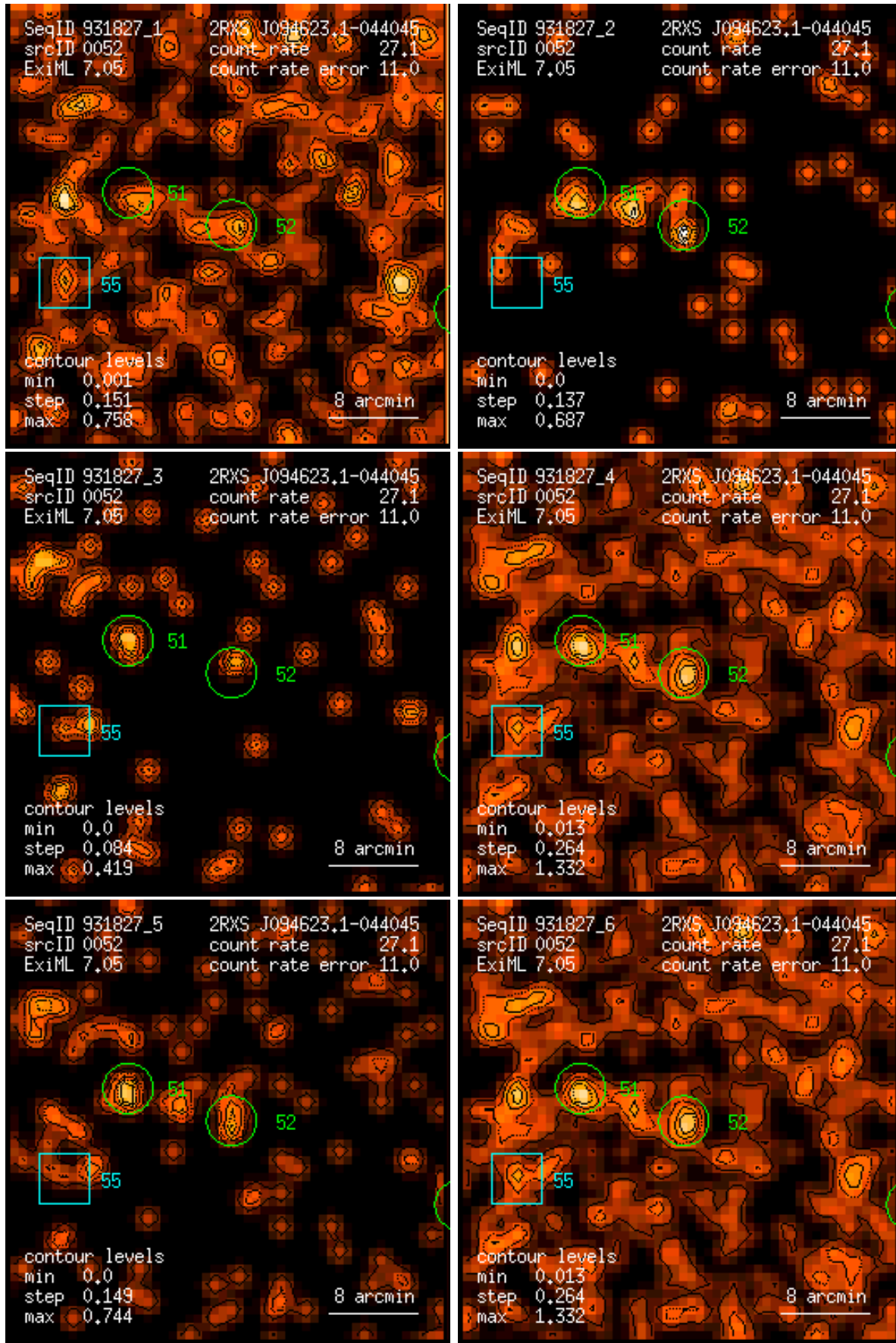
Figure 52: RASS 931827: detection 0052: band rate images, Gaussian filter: (1) PSPC channels 11 – 41, (2) 52 – 90, (3) 91 – 201, (4) 11 – 235, (5) 52 – 201, (6) 11 – 201. Broad band rates in counts/ks. Band rate contour levels in counts/ks/arcmin 2 .
