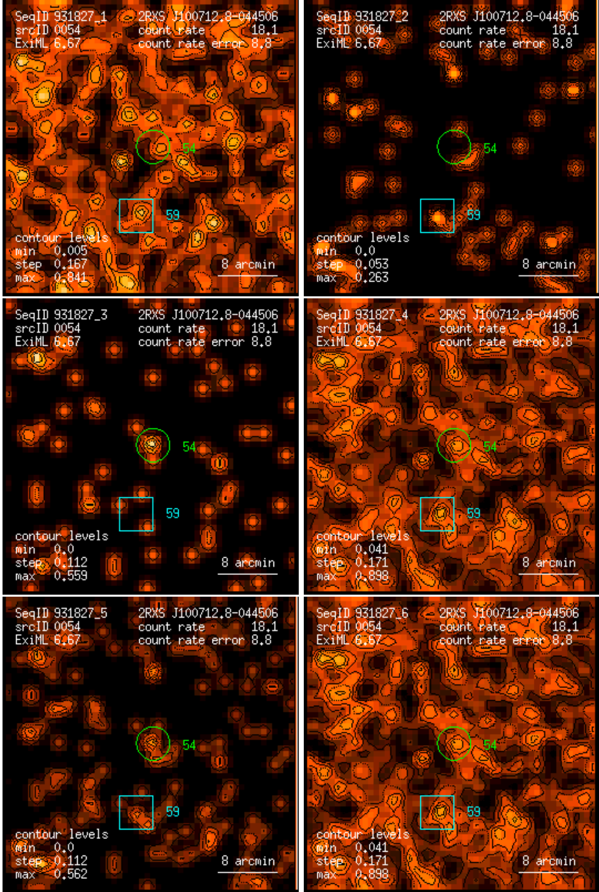
Figure 54: RASS 931827: detection 0054: band rate images, Gaussian filter: (1) PSPC channels 11 – 41, (2) 52 – 90, (3) 91 – 201, (4) 11 – 235, (5) 52 – 201, (6) 11 – 201. Broad band rates in counts/ks. Band rate contour levels in counts/ks/arcmin 2 .
